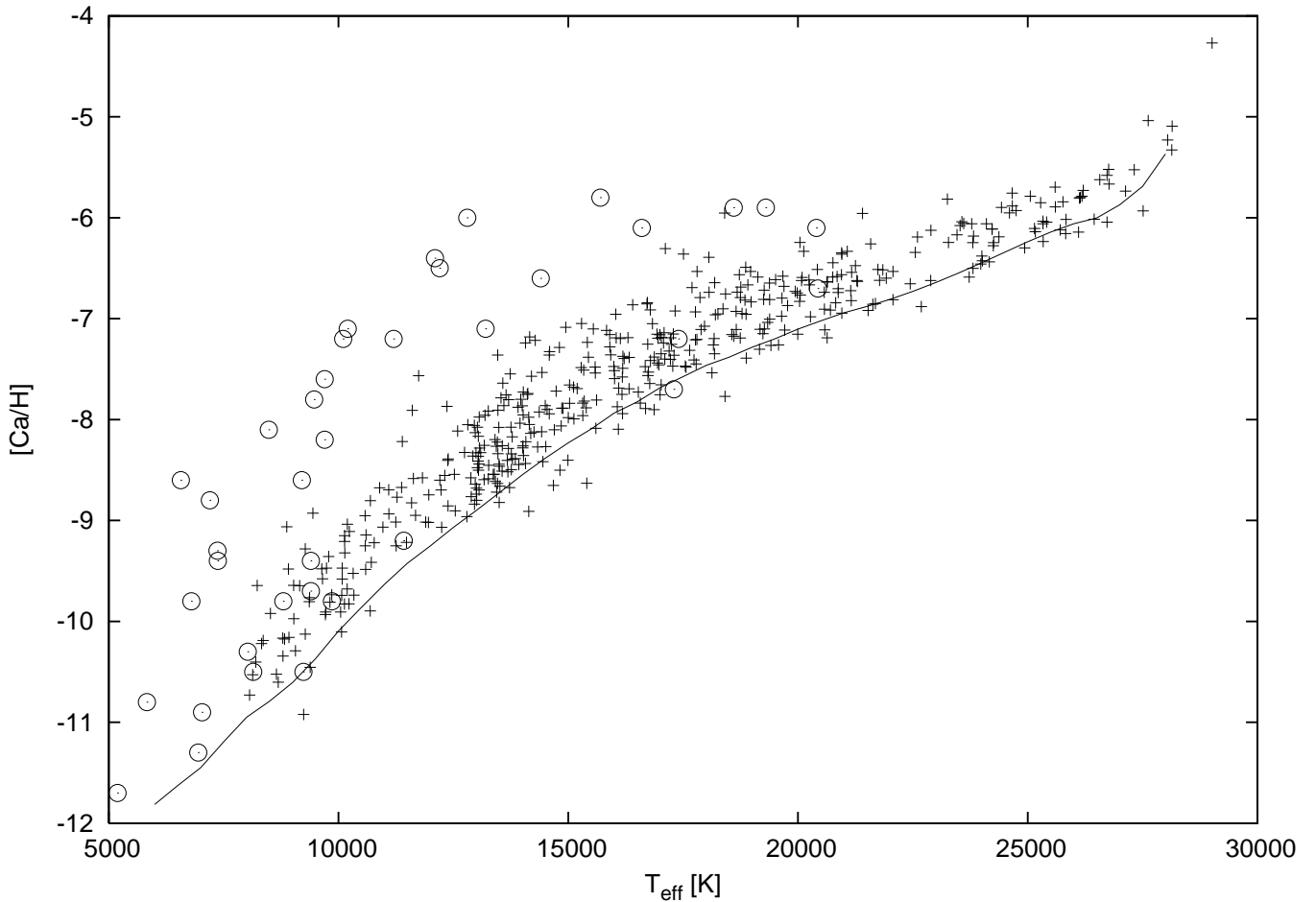
Fig. 1. Logarithmic Ca abundances (circles) and upper limits (crosses) for the combined sample (see text). The continuous line indicates a constant equivalent width of EW=15\text{m}\text{\AA} , taken as observational limit for most objects
