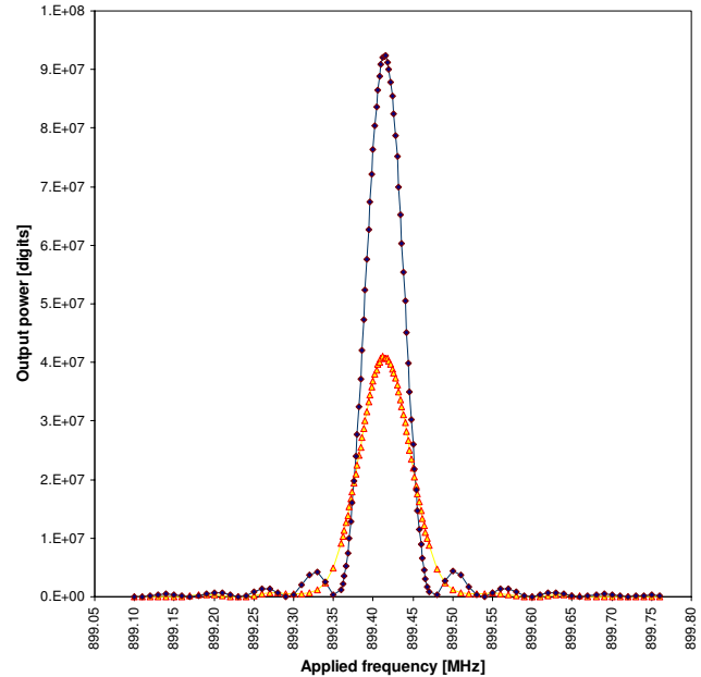
Fig. 4. Filter curve obtained by measuring the output of frequency channel 14736 (899.414 MHz) while a signal generator producing a very narrowband signal at the applied frequency is stepped through the band. The observed output power of the FFT spectrometer in unfiltered mode, corresponding to a boxcar filter with one channel's width, is given with diamonds, the result applying a Kaiser filter is displayed with triangles.
