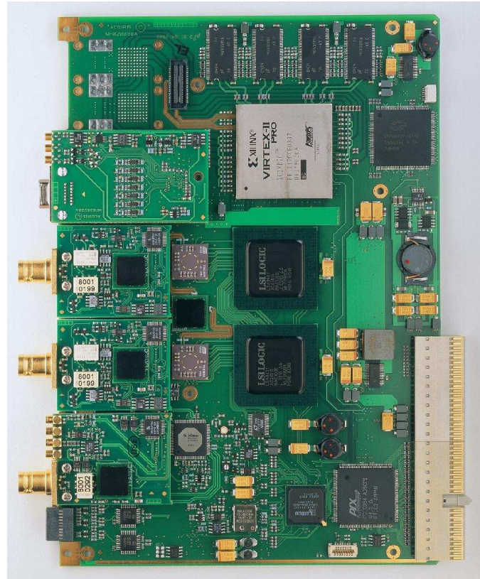
Fig. 1. Board of AC240, the hardware of the FFT spectrometer. On the left, from top to bottom, are the system control interfaces, two analog inputs for the signal at intermediate frequency (SMA connectors will be used in the final version), and an input for a trigger or a clock. The FPGA processing unit is visible in the top center, the PCI bus for data output at the bottom right.
