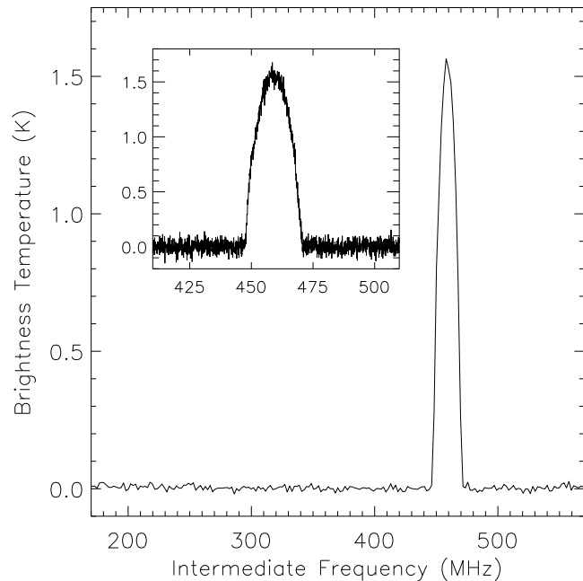
Fig. 6. First light spectrum around the relatively weak CO(2-1) line of the evolved carbon star IRC +10216 observed with the FFT spectrometer for a net on-source time of 57 minutes. The frequency is the intermediate frequency as measured by the spectrometer. To reduce noise, 32 channels are integrated (resolution 1.95 MHz). The insert is an enlargement of the line in full resolution (61 kHz).
