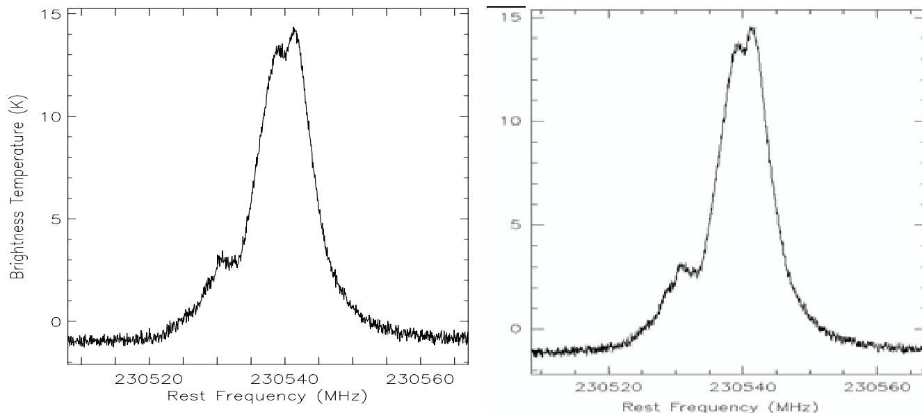
Fig. 7. Left: The CO(1-2) line of the high-mass protostar DR 21K, observed with the FFT spectrometer for a net on-source time of 90 s. Right: A comparable observation with the high-resolution acousto-optical spectrometer of KOSMA.
