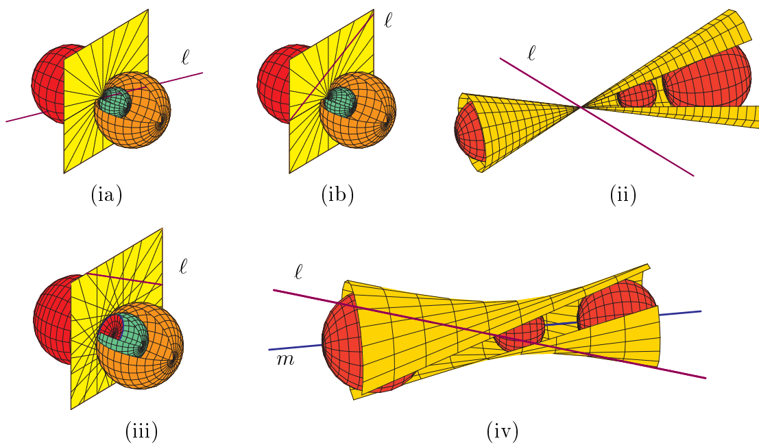
FIGURE 1. The Geometry of Theorem 1.
