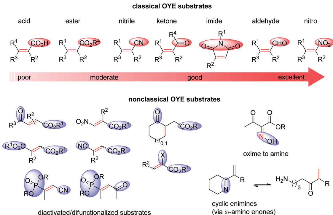
Scheme 2 Classical substrates for Old Yellow Enzymes (OYEs) listed according to reactivity, and nonclassical substrates.
