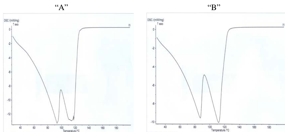
Figure 3: DSC thermogram of native (A) and acetylated (B) acha starches
