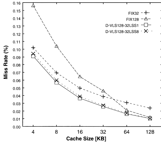
Fig. 9 Miss rate versus cache size.
