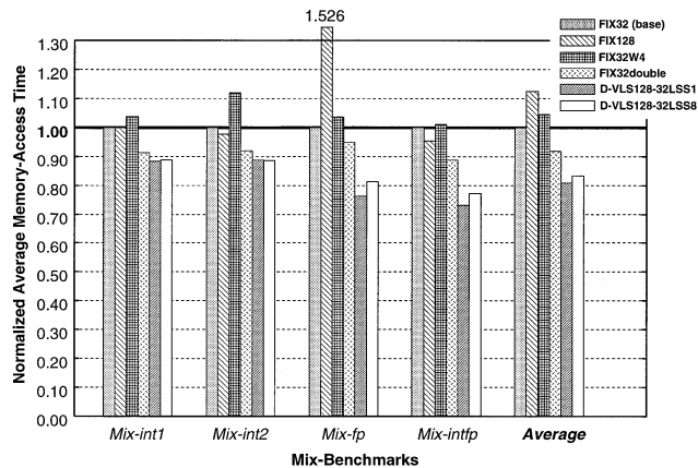
Fig. 8 Average memory-access time for benchmark sets.
