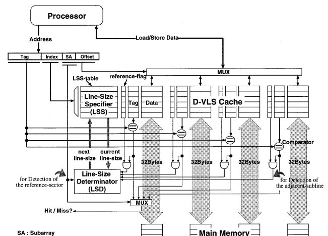
Fig. 3 Block diagram of a direct-mapped D-VLS cache.
