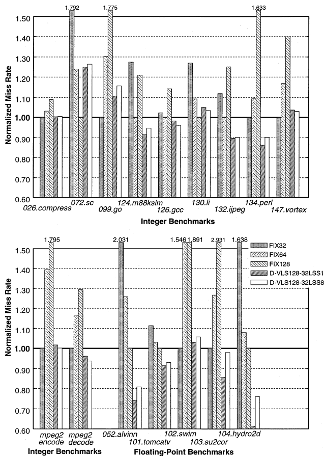
Fig. 5 Miss rates for benchmarks.
