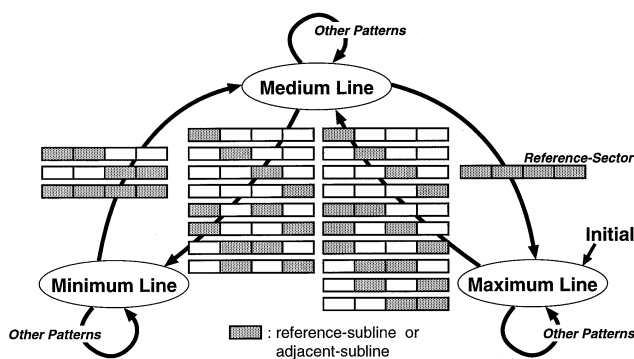
Fig. 4 State transition diagram.
