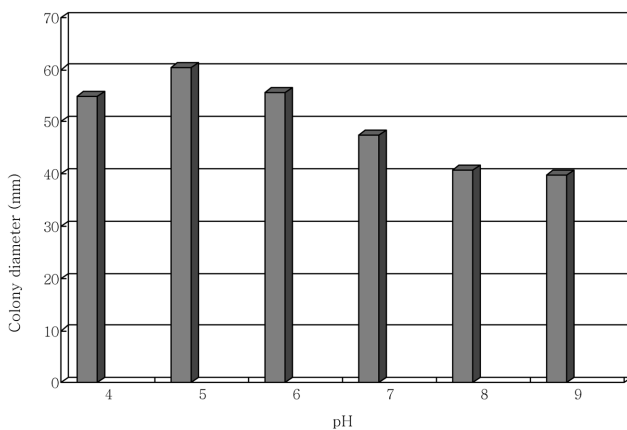
Fig. 1. Mycelial growth of Cystoderma amianthinum on the PDA at different pHs for 20 days of incubation at 25°C.
