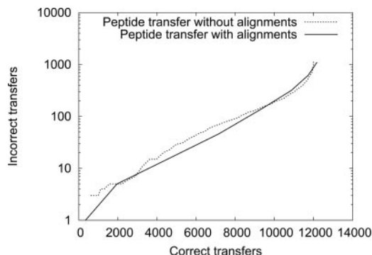
FIG. 6. Correct peptide ID transfer rate against incorrect peptide transfer rate while transferring identifications from time point 30 to time point 0 in yeast whole-cell lysate experiment.
