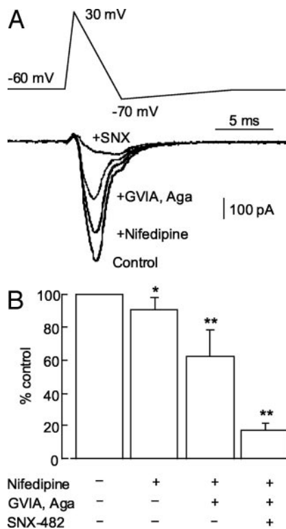
FIG. 4. The \text{Ca}^{2+} currents elicited by APW in neonatal GnRH neurons. The action potential waveform is composed of the 1-msec depolarization phase from -60 mV to 30 mV, the 4-msec repolarization phase from 30 to -70 mV, and the 10-msec afterhyperpolarization phase from -70 mV to -60 mV as shown in A. After control recording, drugs were successively applied as indicated. B, Collective presentation of the effects of drugs. The data for both sexes are combined ( n = 8 ). Aga, Aga-IVA; -, without drug application; +, with drug application. The inhibitory effect of each drug was evaluated by comparing the responses with and without the drug in a paired t test. *, P < 0.05 ; **, P < 0.01 .
