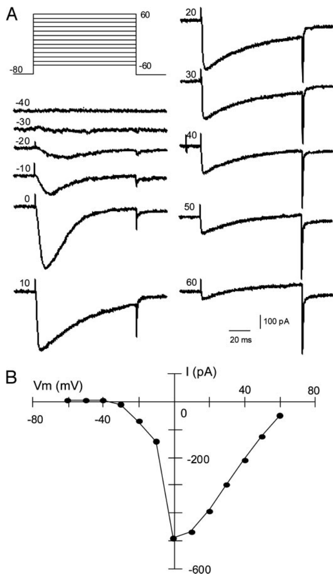
FIG. 2. Voltage-gated Ca 2+ currents in neonatal GnRH neurons. After perforation with amphotericin B, cells were clamped at -80 mV and given 100-msec voltage pulses from -60 to 60 mV in 10-mV steps from a holding potential of -80 mV as shown at the upper left in A. A, Current traces elicited with voltage pulses as indicated at the upper left in each trace. Current traces at -60 mV and -50 mV are not shown. B, IV relationship of the peak currents with the same data as in A.
