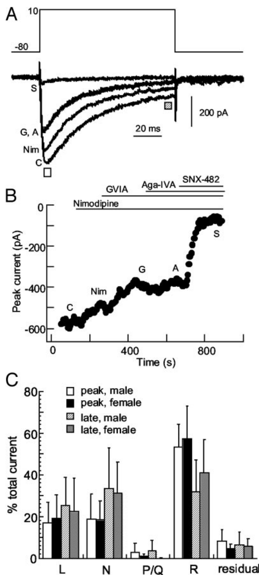
FIG. 3. Pharmacological characterization of the Ca 2+ currents in neonatal GnRH neurons. A, Voltage protocol and the representative current traces. Voltage pulses (10 mV in this cell) were applied from the holding potential of -80 mV at 0.2 Hz. The control trace is labeled C. The current was attenuated by 10 \mu M nimodipine (Nim), 1 \mu M GVIA (G), and 100 nM SNX-482 (S). A concentration of 200 nM Aga-IVA (A) had no effect on the current in this cell. Therefore, traces labeled G and A are overlapped. These traces were taken from the same data for B at time points denoted by C, Nim, G, A, or S. B, Time course of the effect of drugs on the peak Ca 2+ current is shown. Drugs were applied as indicated with horizontal bars. C, The effects of drugs are collectively shown as a percentage of the total current ( n = 11 in males, 14 in females) for the initial peak current (peak) and the late sustained current (late). The late sustained current was measured as the mean current of the last 5 msec of the 100-msec pulse (hatched square in A). The L-type current indicates the current blocked by nimodipine. The N-type current (N) is the current blocked by GVIA. The P/Q-type current (P/Q) is the current blocked by Aga-IVA. The R-type current (R) is the current blocked by SNX-482. Residual indicates the current resistant to all these drugs.
