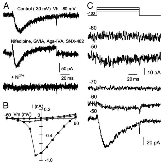
FIG. 7. T-Type current in GnRH neurons. A, The currents were elicited by a -30 mV pulse from the holding potential of -80 mV in neurons around puberty. Combined application of nifedipine (10 \mu M), GVIA (1 \mu M), Aga-IVA (200 nM), and SNX-482 (100 nM) slightly attenuated the peak amplitude of the current. This remaining current was almost completely blocked by 50 \mu M Ni 2+ (lower trace). B, IV relationship of the peak current in the control (■); with nifedipine, GVIA, Aga-IVA, and SNX-482 (○); and with the addition of Ni 2+ (●). C, The voltage pulses to -70 , -60 , and -50 mV were given from the holding potential of -100 mV at 0.2 Hz, as shown at the top. The upper two current traces are from the neonatal neuron (male, 3 d old). The current at -70 mV is not shown. The lower three traces are from the neuron around puberty (female, 35 d old). The numbers at the upper left in each trace indicate the amplitude of voltage pulses. For clarity, the currents in C were filtered at 500 Hz.
