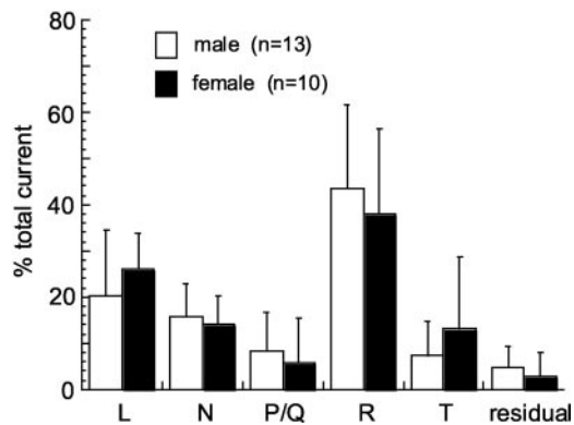
FIG. 6. Pharmacological characterization of the Ca 2+ currents in GnRH neurons around puberty. Effects of drugs are collectively shown as a percentage of the total current for the peak current. The L-type current (L) was the current blocked by 10 \mu M nifedipine; the T-type current (T) was the current resistant to nifedipine, GVIA, Aga-IVA, and SNX-482 and blocked by 50 \mu M Ni 2+ . Other currents are the same as in Fig. 3. The experimental procedure is the same as for the neonatal neurons.
