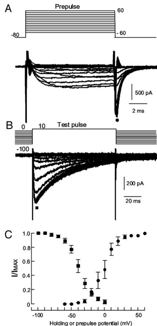
FIG. 5. Activation and steady-state inactivation of the R-type \text{Ca}^{2+} current in neonatal GnRH neurons. A, The upper panel shows the voltage protocol for the activation. The holding potential was -80 mV. Ten-millisecond prepulses of -60 to 60 mV were applied, and the tail currents at -80 mV were measured as indicated ( \bullet ). B, Holding potentials varied from -100 to 0 mV, and the currents elicited by the test pulse ( 10 mV) were measured as indicated ( \blacksquare ). C, Activation ( n = 4 ) and steady state inactivation ( n = 10 ) are shown. The data for both sexes were combined. The half-activation voltage was 0 mV, and the half-inactivation voltage was -39 mV.
