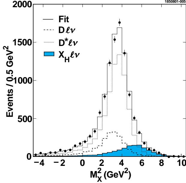
FIG. 1. Measured \widetilde{M}_X^2 distributions, for background-corrected data (points), Monte Carlo (solid line), and the three components of the Monte Carlo: B \rightarrow D\ell\nu (dashed), B \rightarrow D^*\ell\nu (dotted), B \rightarrow X_H\ell\nu (shaded). The normalization of each component is derived from a fit to the data.
