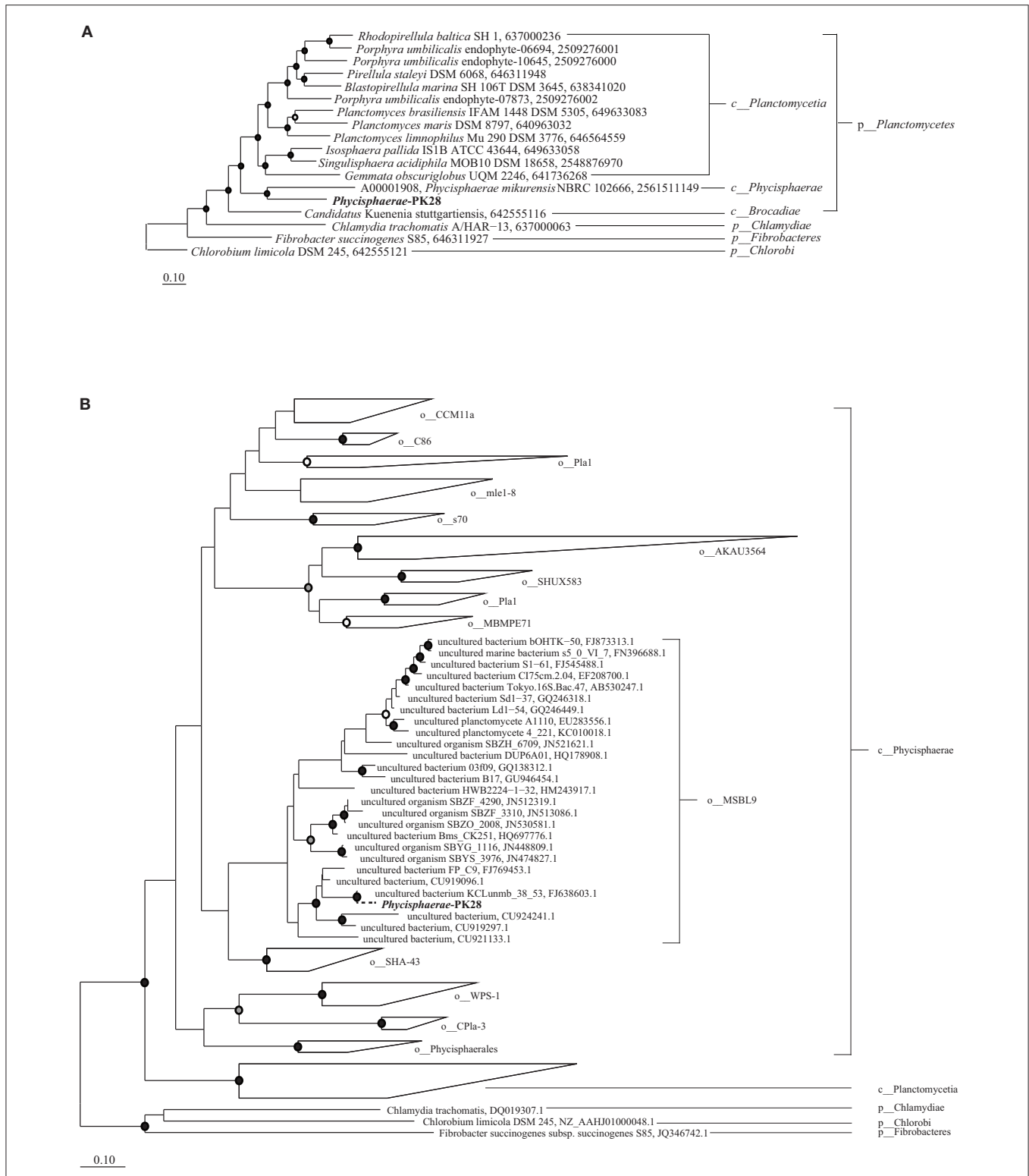
FIGURE 4 | Maximum likelihood phylogenetic trees showing the placement of Phycisphaerae -PK28 within the phylum Planctomycetes using (A) a concatenated set of 83 bacterial single-copy marker genes and (B) 16S rRNA gene sequences from Phycisphaerae -PK28 and members of the phylum Planctomycetes . These analyses place Phycisphaerae -PK28 into the order MSLB9 within the class Phycisphaerae . NCBI accession numbers and IMG genome IDs are listed to the right of each sequence. In both trees, white, gray, and black circles represent nodes with 70–80%, 80–90%, and >90% bootstrap support values respectively. For the concatenated marker gene tree, members of the phyla Chlamydiae, Fibrobacter, and Chlorobi were used to root the tree.
