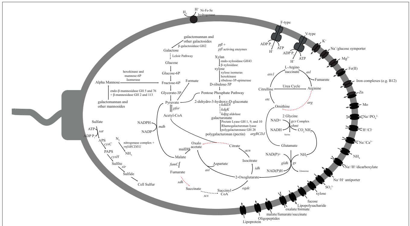
FIGURE 6 | Metabolic reconstruction of the Phycisphaerae -PK28 population genome. Sugar polymers such as galactomannan (guar), xylan (hemicellulose), and polygalacturonan (pectin) may be degraded and directed toward glycolysis for energy production. The pyruvate generated through glycolysis is likely to be converted to formate by pyruvate-formate lyase. Nitrogen and sulfur could be acquired through nitrogen fixation and assimilatory sulfate reduction. Abbreviations used: fumC , fumarate hydratase; sdh , succinate dehydrogenase; scs , succinyl-CoA synthetase; ogdc , oxoglutarate dehydrogenase complex; idh , isocitrate dehydrogenase; can , citrate hydro-lyase; cs , citrate synthase; ass1 , argininosuccinate synthase; otc , ornithine transcarbamylase; arg , arginase; asl , argininosuccinate lyase; pfor , pyruvate-ferrodoxin oxidoreductase; mdh , malate dehydrogenase; pfl , pyruvate-formate lyase; mf , Rnf electron transport complex; ast , aspartate transaminase; gs , glutamate synthetase; gldh , glutamate dehydrogenase; gcs , glycine cleavage system; shmt , serine hydroxymethyltransferase; argB , acetylglutamate kinase; argC , N-acetyl-glutamate semialdehyde dehydrogenase; argD , N-acetylornithine aminotransferase; argJ , arginine biosynthesis bifunctional protein; sat , sulfate adenyltransferase; cysC , adenylsulfate kinase; cysH , phosphoadenylsulfate reductase; and sir , assimilatory sulfite reductase.
