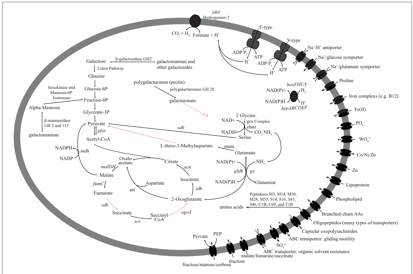
FIGURE 7 | Metabolic reconstruction of the Aminicenantes -PK28 population genome. The sugar polymers galactomannan (guar) and polygalacturonan (pectin) may be degraded. Galactomannan is likely to be directed toward glycolysis for energy production. Although polygalacturonases were identified, it is not clear how Aminicenantes -PK28 processes galacturonate. Several peptidases involved in the degradation of oligopeptides were identified, including family M23, which is involved in the lysis of bacterial cells. These findings suggest that Aminicenantes -PK28 may scavenge non-viable cells. Abbreviations used: fumC , fumarate hydratase; sdh , succinate dehydrogenase; scs , succinyl-CoA synthetase; ogdc , oxoglutarate dehydrogenase complex; idh , isocitrate dehydrogenase; can , citrate hydro-lyase; cs , citrate synthase; mdh , malate dehydrogenase; pfor , pyruvate-ferrodoxin oxidoreductase; ast , aspartate transaminase; gs , glutamate synthetase; gldh , glutamate dehydrogenase; gcs , glycine cleavage system; shmt , serine hydroxymethyltransferase; sdh , serine dehydrogenase; fdh , formate dehydrogenase.
