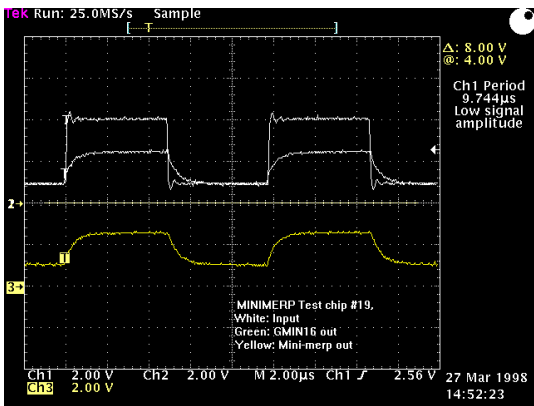
Figure 7. Propagation delay test on a miniMERP circuit. Bottom curve is the output, as the smaller of the two inputs.
