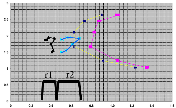
Figure 5 (a). A simulation result showing the required trapezoidal membership functions for discrimination of two targets r1 and r2 .
