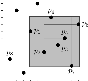
Figure 3: A pin sequence.
