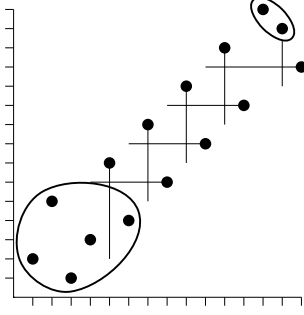
Figure 4: The element \beta_5 in the basis of \text{Av}(25134) \wr \text{Av}(321) .
