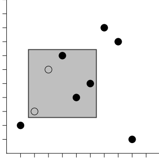
Figure 2: The minimal block \text{mb}(\pi; 2, 3) in \pi = 236745981 .
