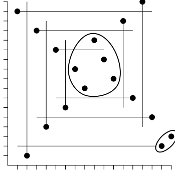
Figure 6: The basis element \beta_3 in \text{Av}(31542) \wr \text{Av}(3412, 2413) .
