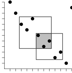
Figure 1: Two intervals and their intersection.
