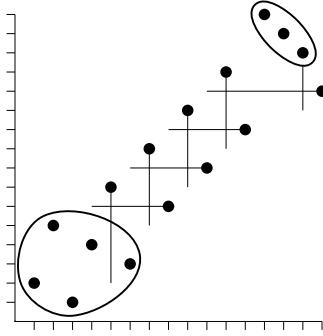
Figure 5: The element \beta_5 in the basis of \text{Av}(25143) \wr \text{Av}(4321, 4123) .
