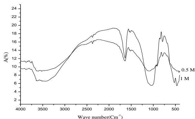
Fig. 2. FTIR spectrum of acid activated bentonites.
