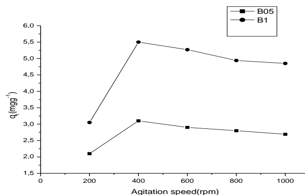
Fig. 4. Effect of agitation speed on the sorption of Zinc by both activated clay B1 and B05. Conditions: pH = 4.5; initial concentration of Zn(II) = 6.7 \text{mg}\cdot\text{L}^{-1} and T = 25 °C.
