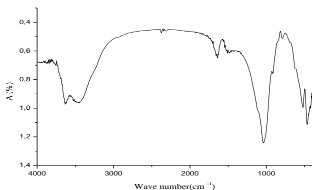
Fig. 1. FTIR spectrum of raw bentonite.
