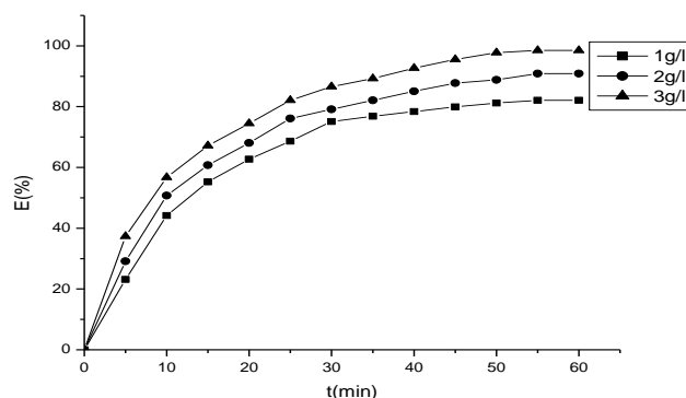
Fig. 5. Effect of dosage of B1 activated bentonite on the sorption of Zinc. Conditions: pH = 4.5; initial concentration of Zn(II) = 6.7 \text{mg}\cdot\text{L}^{-1} and temperature = 25 °C.
