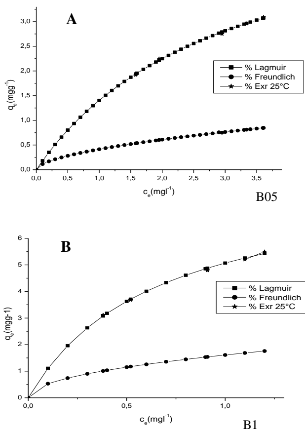
Fig. 8. Sorption isotherms for Zinc onto activated bentonites. Conditions: pH = 4.5; agitation speed = 400 rpm; agitation time = 60 min and temperature = 25 °C.
