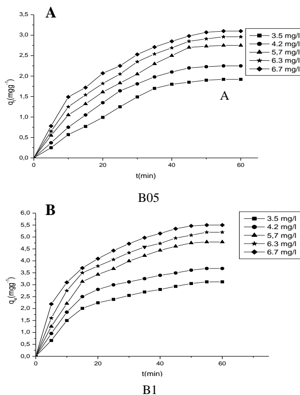
Fig. 3. Effect of contact time on Zn (II) metal ion adsorption by B05 (A) and B1 (B) for different initial Zn (II) ions concentration. Conditions: pH = 4.5; adsorbent dose = 1 \text{g}\cdot\text{L}^{-1} ; agitation speed = 400 rpm and T = 25 ^{\circ}\text{C} .
