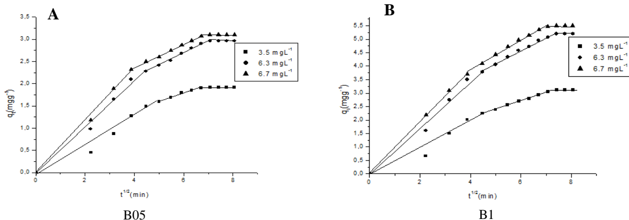
Fig. 7. Intraparticle diffusion plot for Zn (II) adsorption onto acid activated bentonites; Condition: pH = 4.5; agitation speed = 400 rpm and T = 25 °C.
