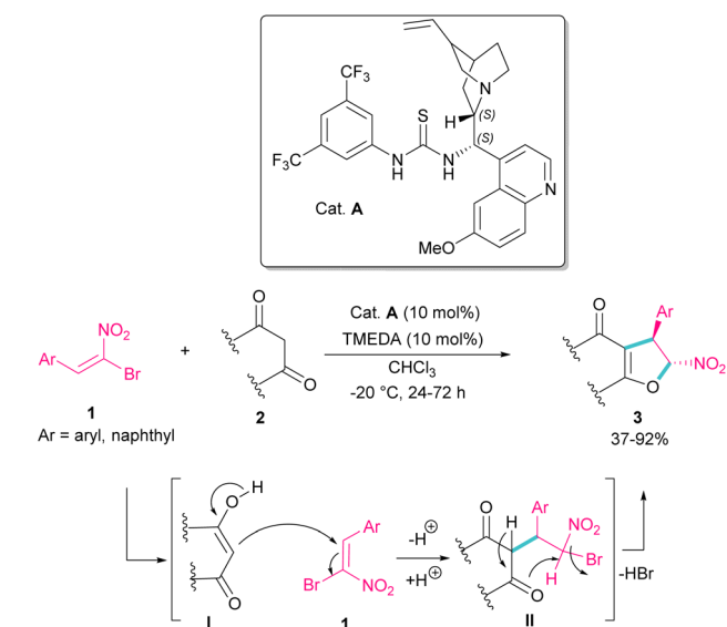
Scheme 2 Organocatalysis reaction of ( E )- \beta -bromonitrostyrenes with 1,3-dicarbonyl compounds.
