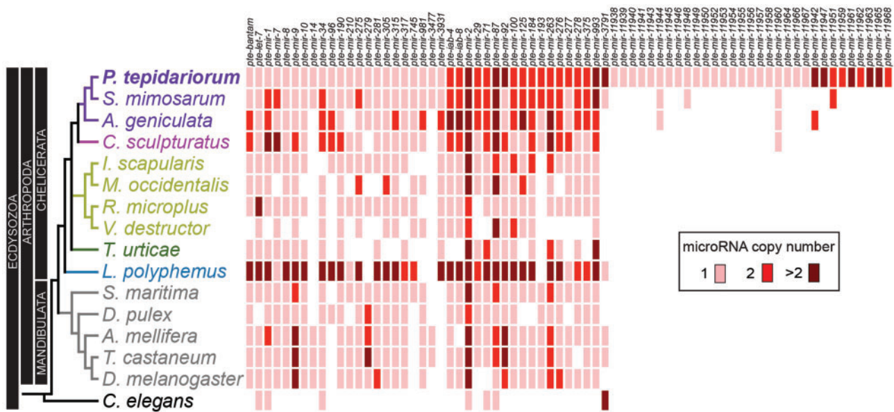
FIG. 2. —MicroRNA family copy number in P. tepidarium and other ecdysozoans. Presence of P. tepidarium single-copy and multicopy microRNA families in other spiders (purple), scorpions (magenta), horseshoe crab (blue) parasitiformes (green), acariformes (dark green), mandibulates (gray), and a nematode (black). The spiders, the scorpion, and the horseshoe crab all display large numbers of multi-copy microRNA families relative to other species.
