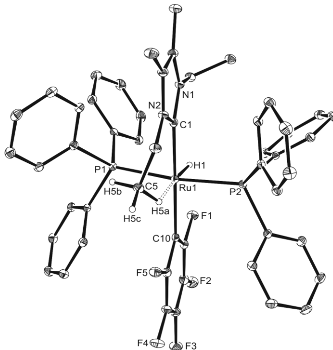
Fig. 3 Molecular structure of 4 . All hydrogen atoms, except Ru-H and those in the agostic methyl group, are omitted. Ellipsoids are shown at the 30% probability level. Selected bond lengths ( \text{\AA} ) and angles ( ^\circ ): Ru(1)-C(1) 2.060(2), Ru(1)-C(10) 2.160(2), Ru(1)-P(1) 2.3452(6), Ru(1)-P(2) 2.3188(6), P(1)-Ru(1)-P(2) 168.093(19), C(10)-Ru(1)-P(1) 91.56(6), C(1)-Ru(1)-P(2) 89.41(6).
