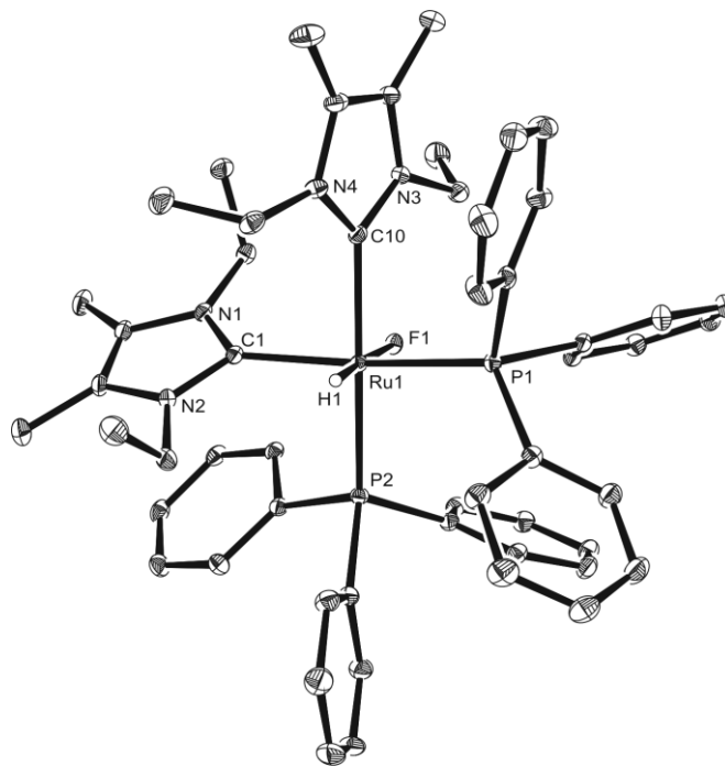
Fig. 1 Molecular structure of 2 . Solvent, minor disordered component and hydrogen atoms (with the exception of the hydride ligand) have been omitted for clarity. Ellipsoids
