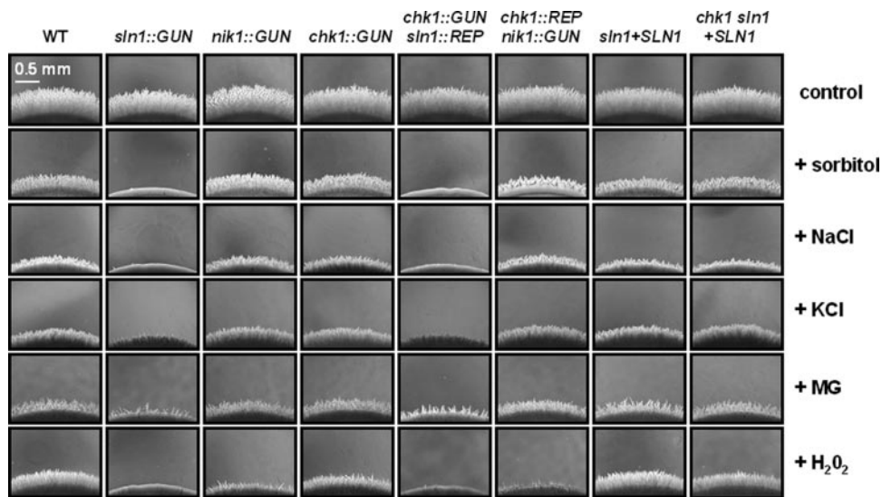
FIG. 6. Pseudohyphal growth abilities of mutants. Cells ( 10^6 ; contained in drops of 5 \mu\text{l} ) of the wild-type strain and representative simple mutants ( sln1::GUN , nik1::GUN , and chk1::GUN ), double mutants ( chk1::GUN sln1::REP and chk1::REP nik1::GUN ), and reintegrant strains ( sln1+SLN1 and chk1 sln1+SLN1 ) were spotted on YCB solid medium supplemented or not with discriminatory concentrations of sorbitol (1 M), NaCl (0.5 M), KCl (0.5 M), MG (15 mM), and \text{H}_2\text{O}_2 (1 mM). Observations were done 48 h after spotting. This experiment was done in triplicate, and pictures present representative structures observed for each sample.
