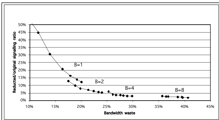
Figure 1. Signalling/Bandwidth trade-off
