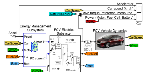
Figure 11: Fuel Cell Vehicle simulation model
