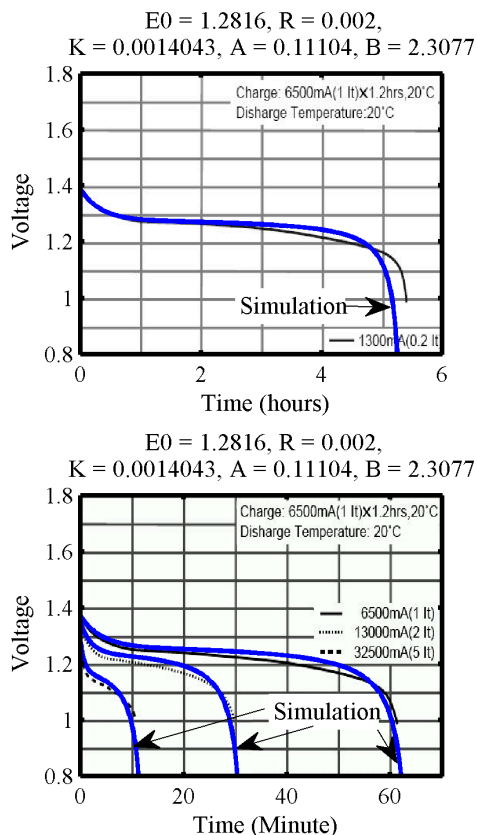
Figure 4: Simulation and datasheet results
