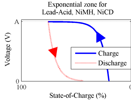
Figure 2: Hysteresis phenomenon
