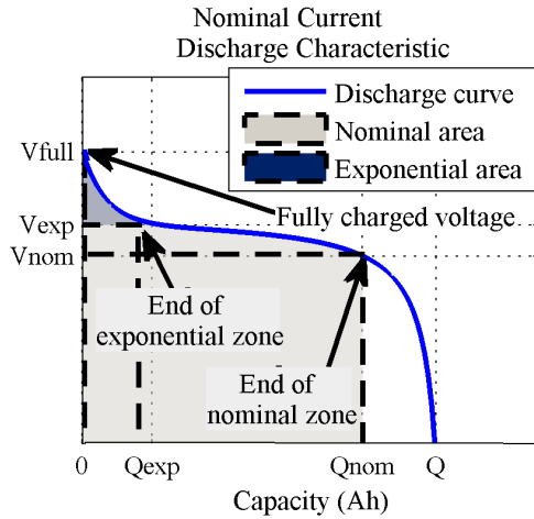
Figure 1: Typical discharge curve
