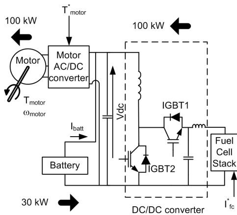
Figure 12: Fuel Cell Vehicle electrical system
