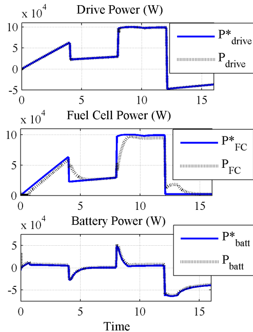
Figure 14: Energy Management System results
