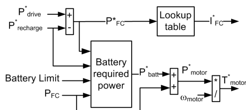
Figure 13: Energy Management System
