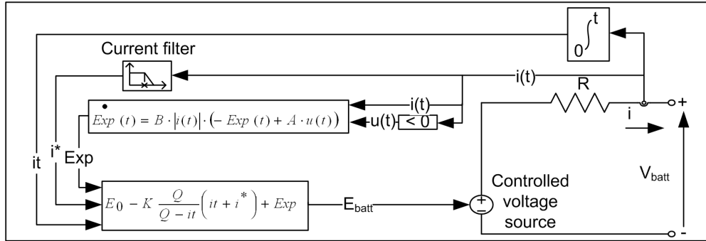
Figure 3: Discharge battery model
