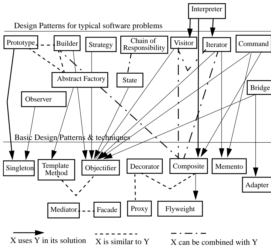
Figure 2.18: The Layered Classification of the Gamma Patterns [Zim94b]
