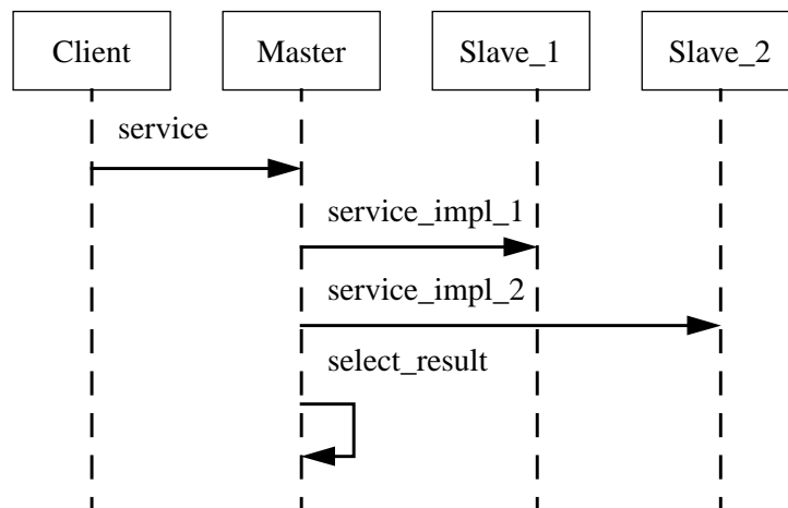
Figure 2.14: Interaction Diagram for the Master-Slave Pattern [Bus94b]
