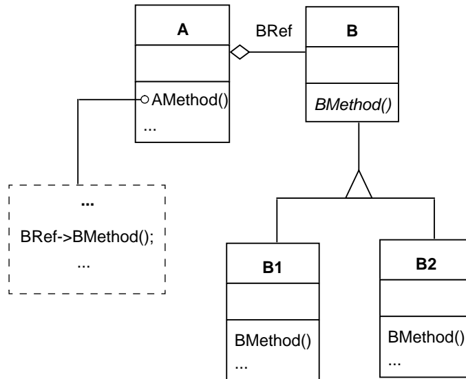
Figure 2.7: Abstract coupling of class A and abstract class B
