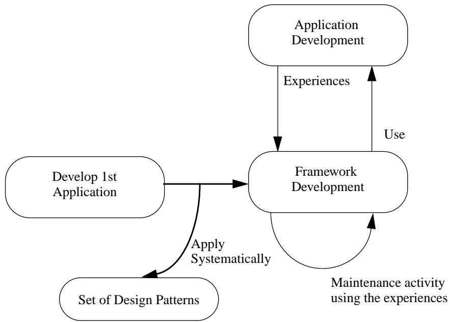
Figure 3.5: Framework Development Process Utilizing Design Patterns
