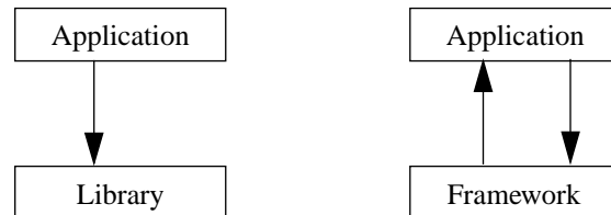
Figure 3.8: The flip-flop of Control
