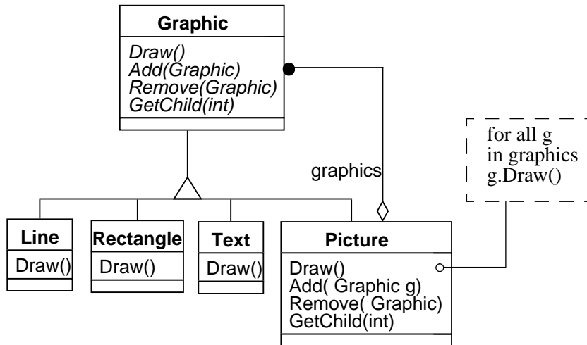
Figure 2.3: The Composite pattern solution
