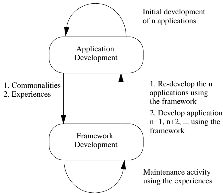
Figure 3.3: Framework Development Process based on Application Experiences
