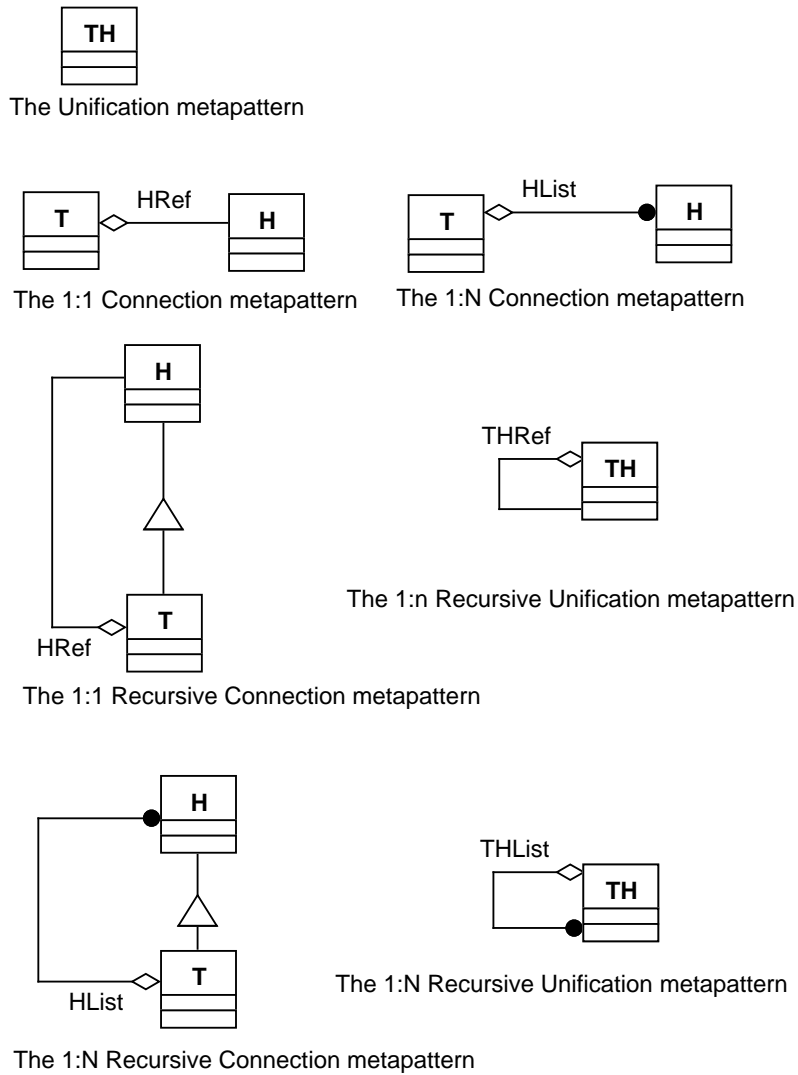
Figure 2.10: The seven metapatterns [Pre94b]
