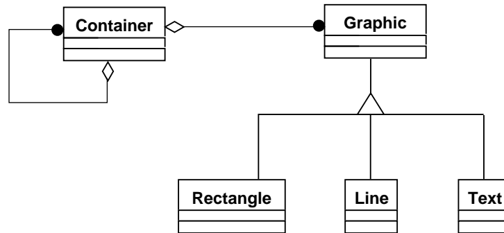
Figure 2.2: The Container Solution
