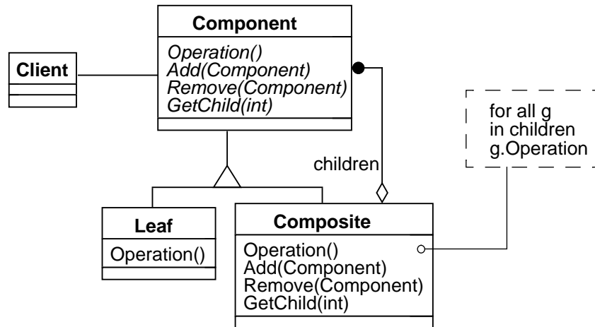
Figure 2.4: The structure of the Composite pattern
