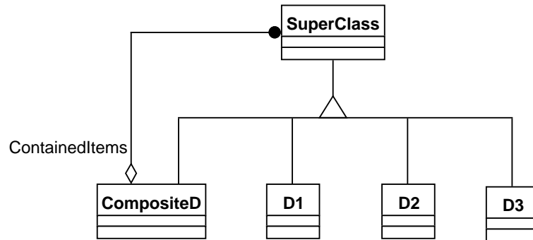
Figure 2.8: A class diagram which enables recursive object structures
