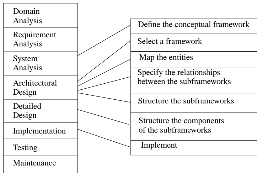
Figure 4.1: Mapping of the activities of the framework-based method to the software process
