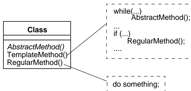
Figure 2.9: Different kinds of methods [Pre94c]
