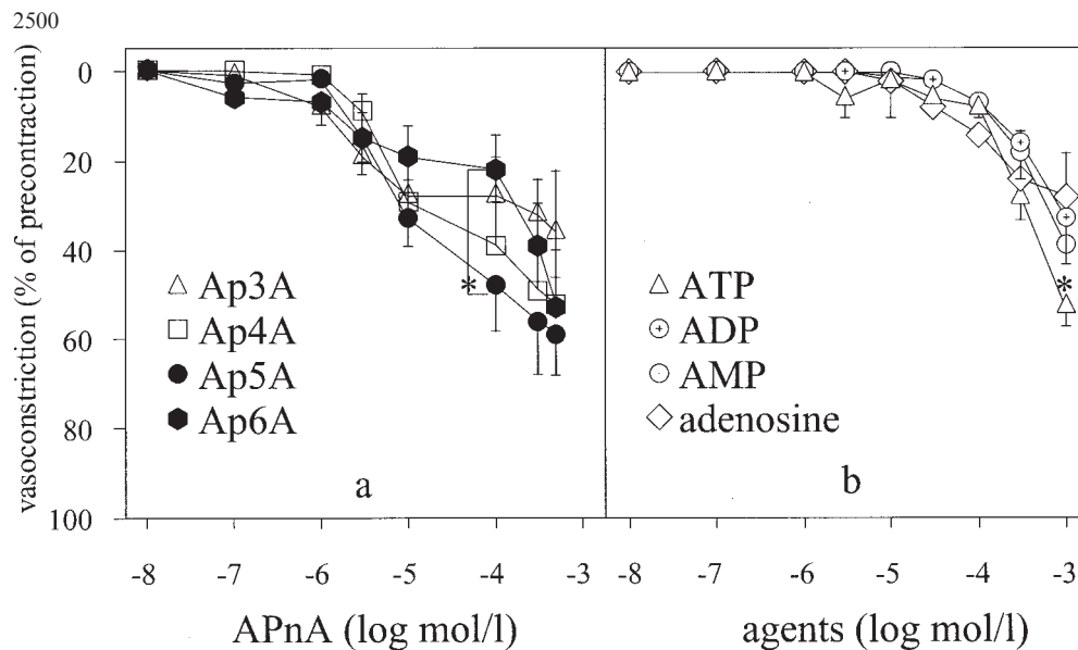
Fig. 3. Relaxing effects of Ap3A, Ap4A, Ap5A and Ap6A (left panel) and of ATP, ADP, AMP and adenosine (right panel) in hRRAs at a phenylephrine (10 µmol/l) pre-contraction. Each point is the mean of 5–7 determinations \pm SEM. * P < 0.05 .
