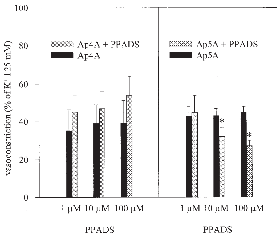
Fig. 4. Contractile effects of Ap4A (100 µmol/l) (left panel) and of Ap5A (100 µmol/l) (right panel) in hRRAs at basal tone presented as a percentage of the response to 125 mmol/l K + (control) as well as contractile effects after pre-incubation with PPADS (1, 10 and 100 µmol/l). Each column represents the mean of 6–10 determinations \pm SEM. * P < 0.05 .
