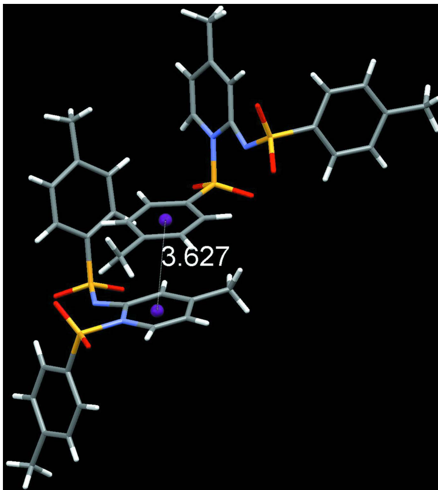
Figure 2 Representation of \pi - \pi stacking in the crystal.
