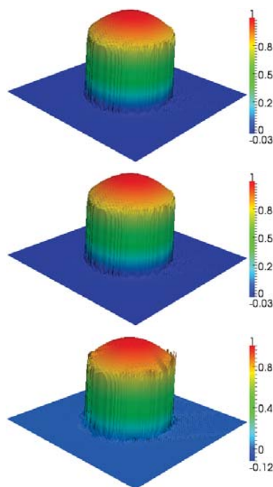
Fig. 3. Hump changing its height, the computed solution with (Q_3^{\text{bubble}}, P_2^{\text{disc}}) and cGP(3) at t = 0.5 , with \mu_0 = 0.01, \mu_0 = 0.1, \mu_0 = 1 ; top to bottom.
