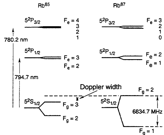
Fig. 1. Partial energy level diagram for Rb 85 and Rb 87 . Within each fine structure level, the hyperfine energy level spacings are drawn to scale.
