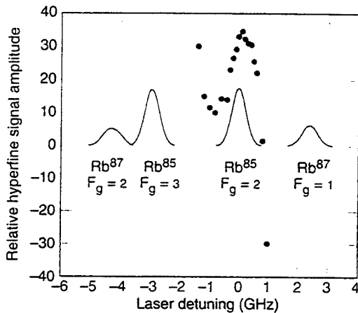
Fig. 5. Resonant nature of the \text{Rb}^{87} hyperfine transition signal with laser tuning about the F_g = 2 \text{Rb}^{85} optical transition. The closed circles correspond to our measurements of the hyperfine resonance amplitude. Contrary to Fig. 4 a positive amplitude corresponds to decreasing absorption, while a negative amplitude corresponds to increasing absorption. The solid curves are simply meant as markers to show the Doppler broadened absorption profiles, and include the influence of the 5^2P_{1/2} excited state hyperfine structure.
