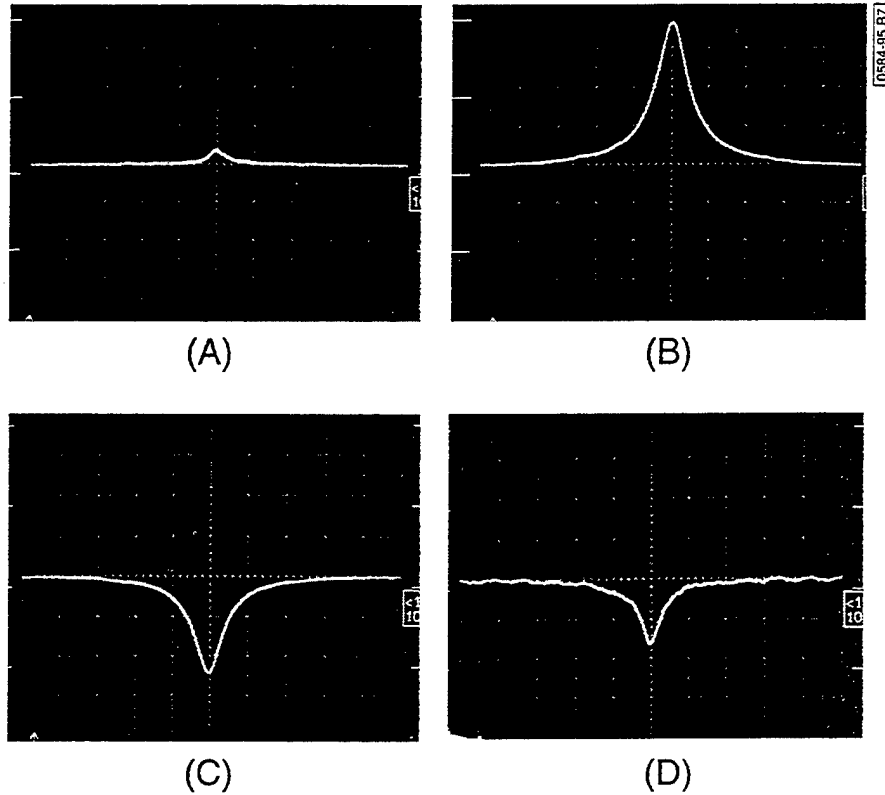
Fig. 4. Oscilloscope traces of the \text{Rb}^{87} 0-0 hyperfine transition lineshapes under varied optical excitation conditions with the probe laser tuned to the \text{Rb}^{87} D_1 [5^2P_{1/2} (F_c = 2) - 5^2S_{1/2} (F_g = 1)] transition. The photocurrent generated by the probe laser's photodiode was detected across 200 k\Omega , and amplified by 200 before being displayed on the oscilloscope: (a) pump laser blocked, 20 mV/cm; (b) pump laser exciting \text{Rb}^{87} atoms out of F_g = 1 hyperfine level, 20 mV/cm; (c) pump laser exciting \text{Rb}^{87} atoms out of F_g = 2 hyperfine level, 20 mV/cm; (d) pump laser exciting \text{Rb}^{85} atoms out of the F_g = 2 hyperfine level, 10 mV/cm.
