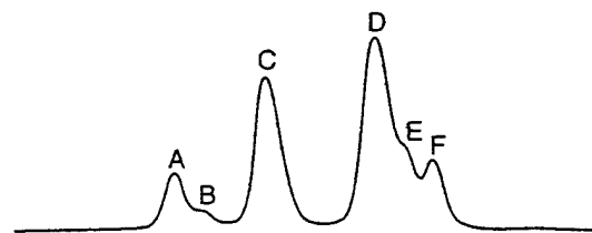
Fig. 3. Probe laser's absorption spectrum for D_1 excitation (i.e., 5^2P_{1/2} \rightarrow 5^2S_{1/2} ): (A) \text{Rb}^{87} (F_e=2) \rightarrow (F_g=1) ; (B) \text{Rb}^{87} (F_e=1) \rightarrow (F_g=1) ; (C) \text{Rb}^{85} (F_e=2, 3) \rightarrow (F_g=2) ; (D) \text{Rb}^{85} (F_e=2, 3) \rightarrow (F_g=3) ; (E) \text{Rb}^{87} (F_e=2) \rightarrow (F_g=2) ; (F) \text{Rb}^{87} (F_e=1) \rightarrow (F_g=2) . Note that the excited state hyperfine splitting in \text{Rb}^{87} is resolved.
