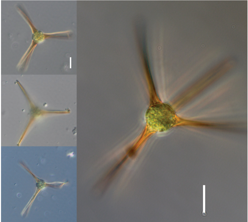
Figures S1. Additional light micrographs showing the morphology of Pachycladella cf. zatoriensis found in Connecticut. Scale bars represent 10 \mu\text{m} .
