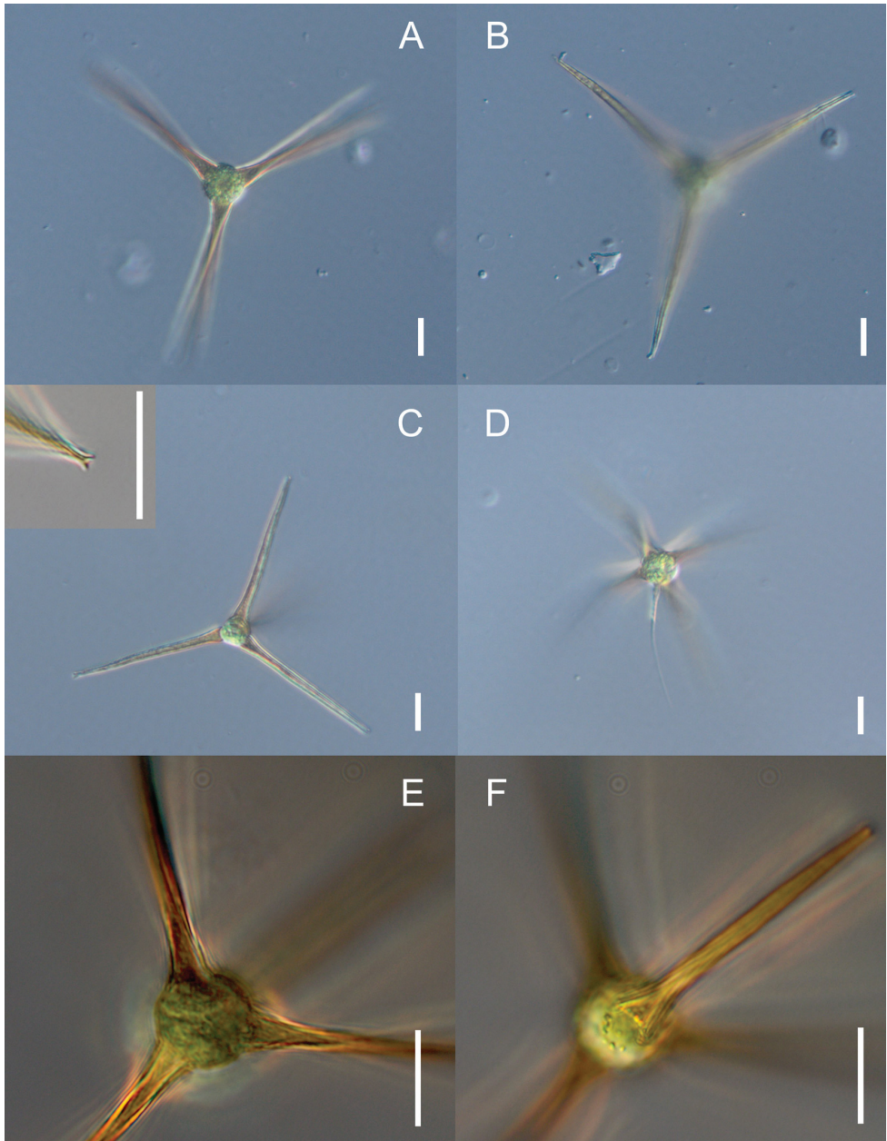
Figure 1. Light micrographs of Pachycladella cf. zatoriensis found in Connecticut. A gross morphology of a vegetative cell B same cell as in A , with focus on process apices C small vegetative cell with a clearly bifurcated process apex (enlarged in the inset) D an unusual cell with a fifth, irregularly placed and colorless appendage E high-magnification micrograph showing the hollow bases of cell wall processes as well as their dark coloration F same cell as in E with focus on the cell surface and attachment of the fourth process. Scale bars represent 10 \mu\text{m} in all images.
