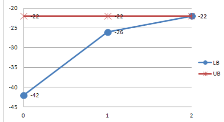
Figure 3: LB & UB vs. Iterations
