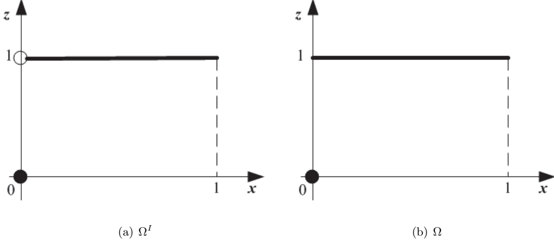
Figure 2: Feasible Sets
