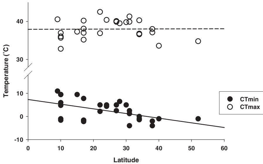
Fig. 3 Changes in CT min and CT max as function of latitude in frogs (data from Brattstrom 1968). CT min (filled circles) is highly negatively correlated with latitude ( p < 0.05 ). CT max (open circles) represent individuals acclimated between 26°C and 30°C (if more than one value existed for a species the mean was taken). CT max is not correlated with latitude ( p > 0.70 ).
