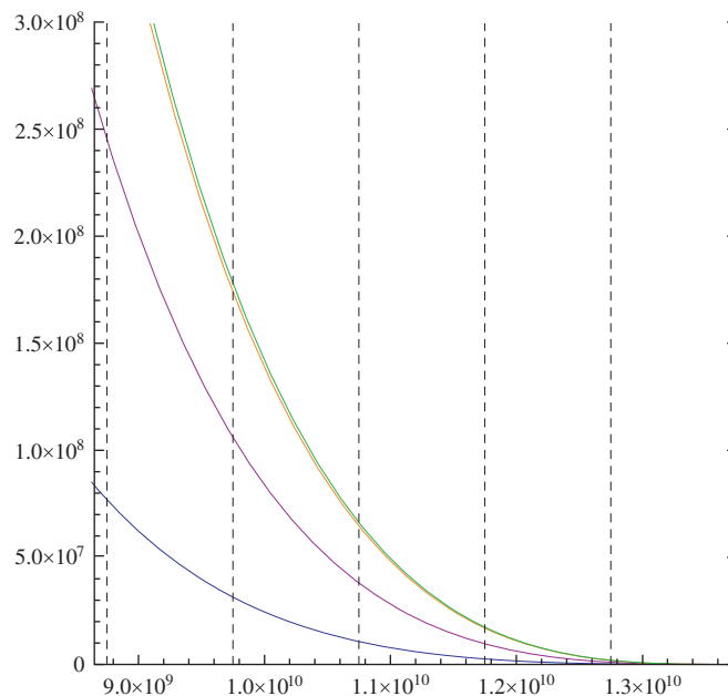
Fig. 5. Number of galaxies that can reach us with speeds of 50% c , 80% c , 99% c and c , from different starting moments.
