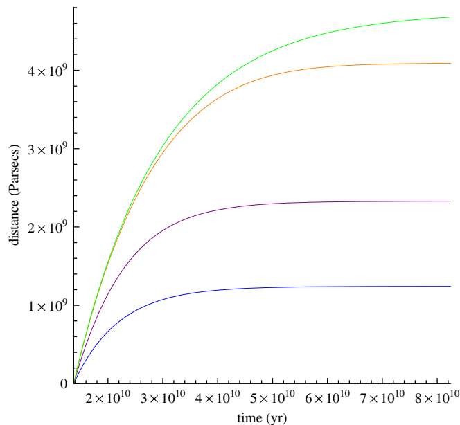
Fig. 4. Distance reached by probes with speeds of 50% c , 80% c , 99% c and c , in comoving coordinates.
