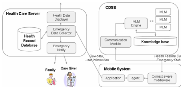
Fig. 5 The process emergency management service
