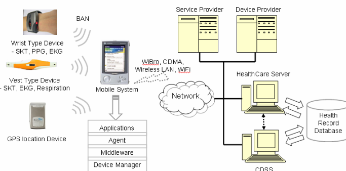
Fig. 2 U-Healthcare infrastructure
