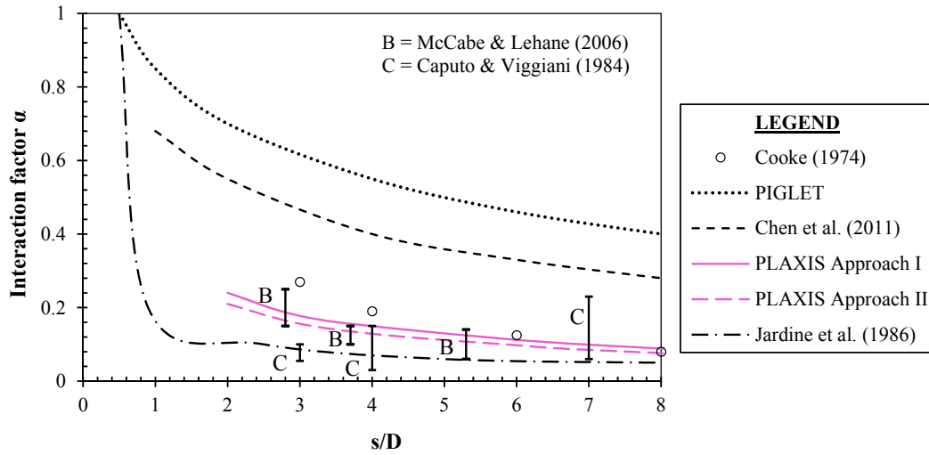
Fig. 5 Comparison of interaction factor predictions determined using Approaches I and II
