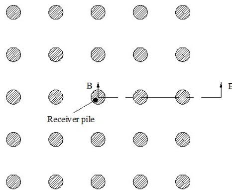
Fig. 7 Cross-section of 25-pile group
