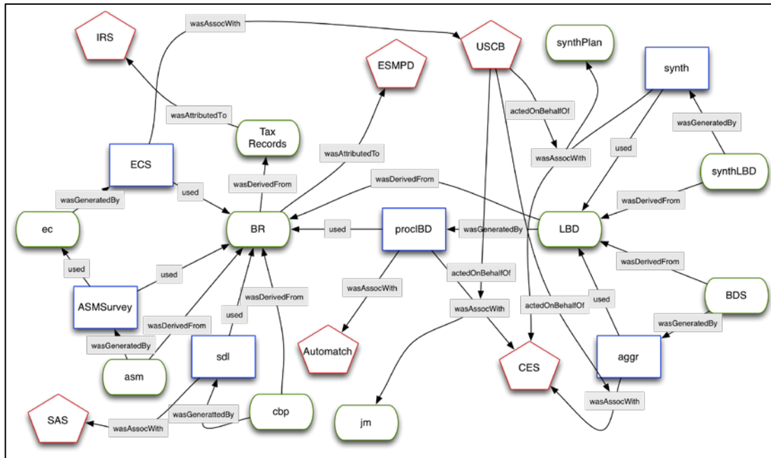
Figure 1. Longitudinal Business Database (LBD) provenance graph
