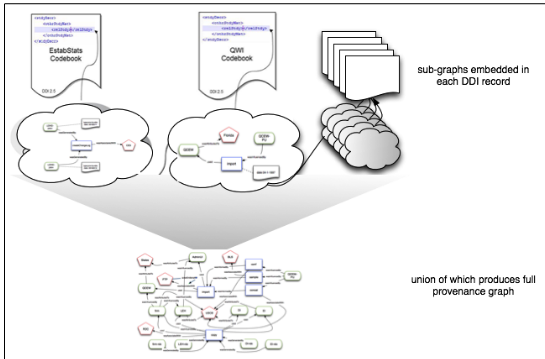
Figure 3. Storing provenance subgraphs related to a given resource within the <relStudy> element in the corresponding DDI metadata. That subgraph links, by resource, to other subgraphs located in other codebooks and ancillary entities (e.g., plans, ages) to allow dynamic generation of the entire provenance graph.
