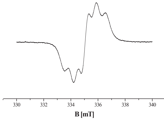
Figure 14. EPR spectrum of DPPH recorded with low microwave power of 2.2 mW. B is the induction of magnetic field.
