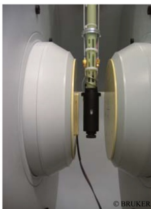
Figure 5. Electromagnet and the resonance cavity of CW-EPR spectrometer produced by Bruker BioSpin GmbH.
