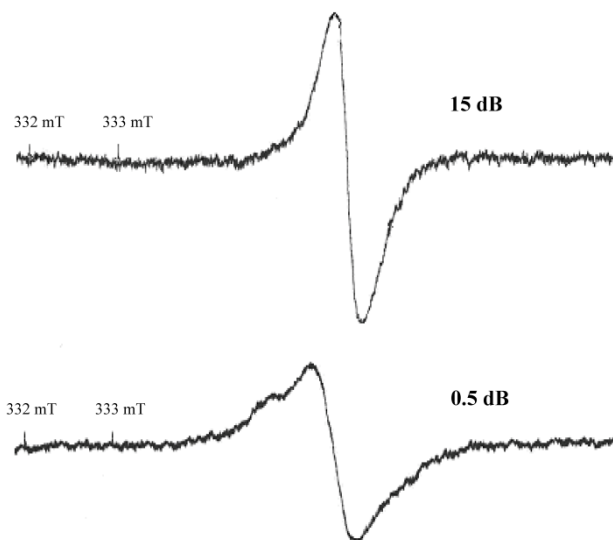
Figure 12. EPR spectra with signals of pheomelanin in Cladosporium cladosporioides recorded with different micro-waves. The melanin samples were studied in paper [52].
