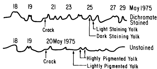
FIGURE 6. Yolk profiles of a single Bar-tailed Godwit egg. Above is the dichromate-stained half of the yolk and below is the unstained half. The arrows indicate a crack that was found after the yolk was cut in half; this crack extended into both halves of the yolk and was used as an additional reference mark. Note correlations between some of the pigmented areas and peaks on the dichromate-stained half. Because darkly staining material (dichromate stain) is laid down during the day, it is concluded that most of the natural pigments of this yolk were ingested during the early morning.
