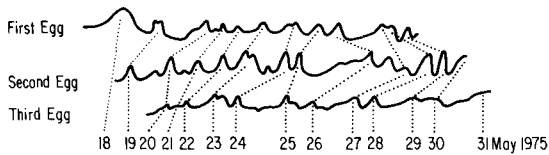
FIGURE 4. Yolk profiles of three Bar-tailed Godwit eggs which had been laid before the nest was discovered. By examination of these stained slices and others that are not stained, the sequence of laying was deduced (see text). The widths of the rings on 24–28 May 1975 in the three eggs were variable, and the profiles appear confusing. Direct observation of ring properties (which are not apparent in yolk profiles) such as color, texture and yolk granule size, however, left little doubt that the sequence was correct.
