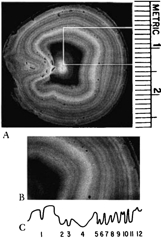
FIGURE 1. A. Photograph of a cross section of a dichromate-stained Bar-tailed Godwit yolk. This yolk required 12 days for formation. The curving of the rings toward the center of the yolk on the left side of the photograph was caused by the neck of the latebra—a structure resulting from non-uniform yolk deposition in the region of the blastodisc. Spots on the yolk are gas bubbles. This particular egg was not degassed completely. B. An enlargement of the outlined part of A showing part of the yolk from the center (left side of the photograph) to the outside. C. The hand-drawn profile represents dark-staining yolk as peaks and pale-staining yolk as valleys. Numbers indicate the days of yolk formation.
