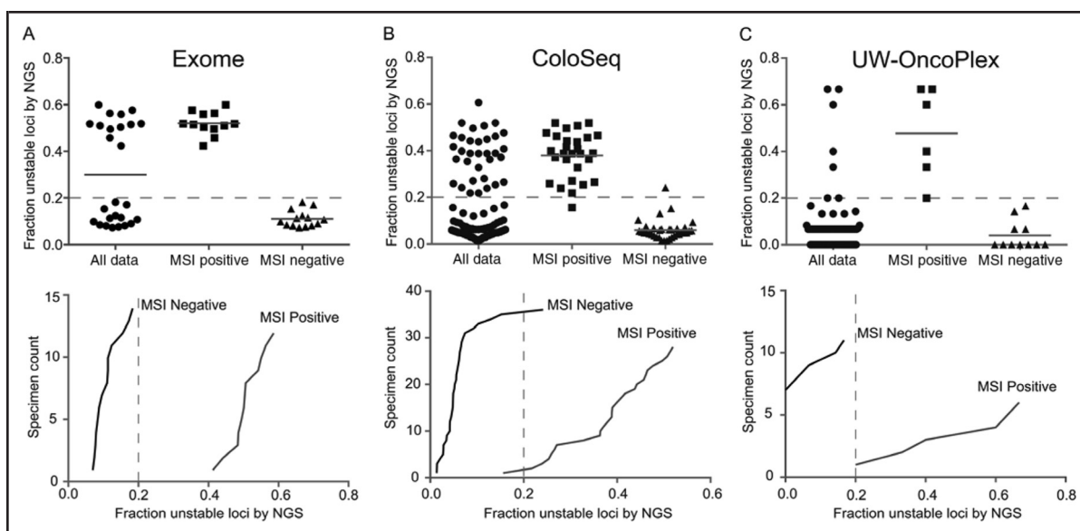
Fig. 2. Fraction of unstable microsatellite loci identified by NGS predicts MSI status.
