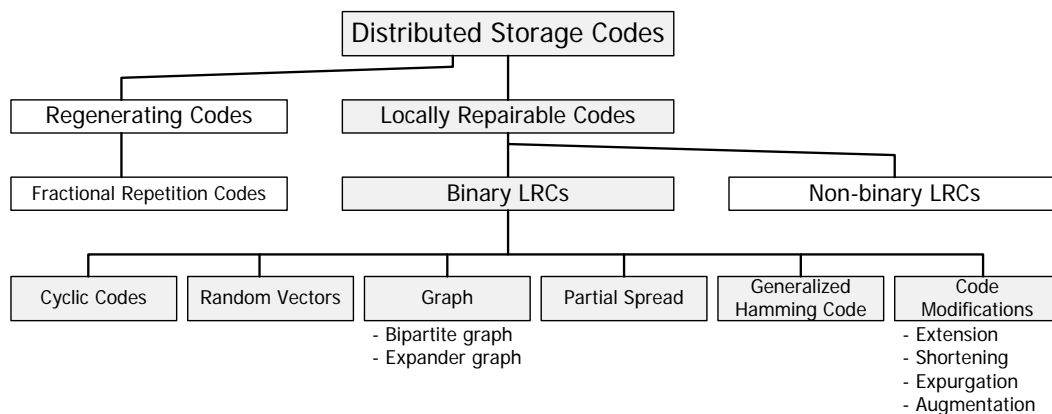
Figure 1. Classification of binary locally repairable codes.
