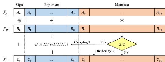
Figure 1: Multiplication of floating point F_A and F_B .
