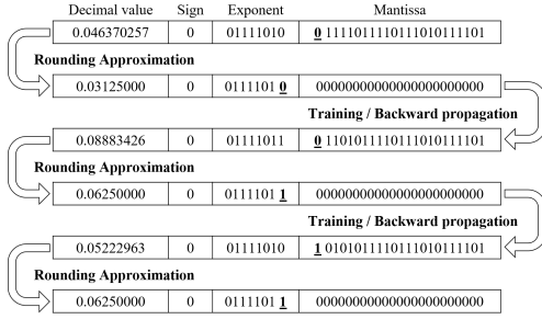
Figure 3: Training procedure for a floating-point filter weight.
