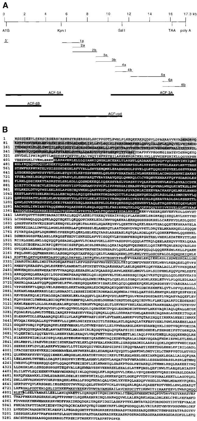
Figure 1. Mouse ACF7. (A) The composite full-length cDNA of mACF7 is 17.3 kb. Fine lines represent RACE-PCR clones and bold lines stand for long-range PCR products. Clone names are shown above each line. The putative start codon (ATG), stop codon (TAA), and unique restriction endonuclease recognition sites, Kpn I and Sal I, used for the construction of full-length mACF7 are indicated. (B) Deduced amino acid sequence of mACF7. The NH 2 -terminal ABD is shaded in gray and the globular plakin-like domain is shaded in black with white letters. The rod domain of mACF7 is made up of 23 spectrin repeats and the corresponding amino acid sequence is boxed.
