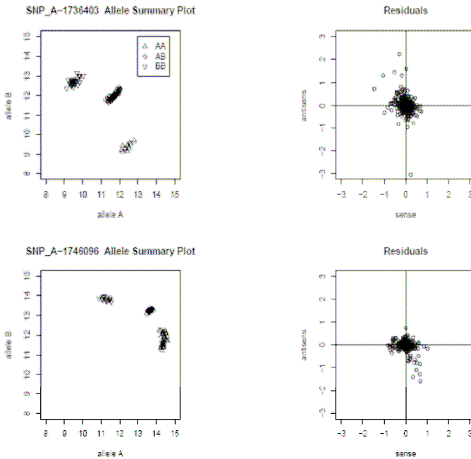
Figure 1 – Side-by-side Allele Summary Plot and Residual Plot for two typical SNPs in the Mapping 100K - Xba set
