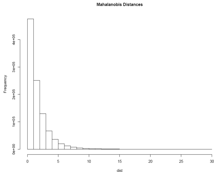
Figure 2 – Histogram of minimum Mahalanobis distances pooled over 5,000 SNPs
