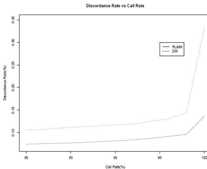
Figure 4 – Percentage of calls discordant with HapMap versus Call Rate for RLMM and DM ( n=11,446 SNPs).
