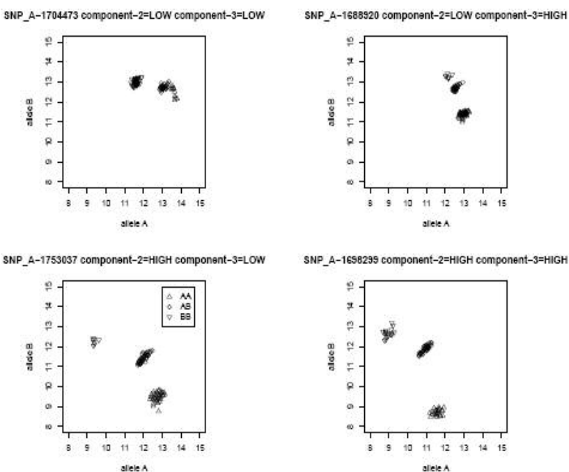
Figure 3 – Allele summary plots of SNPs whose means have difference combinations of HIGH and LOW values of the second and third principal components of the mean vectors
