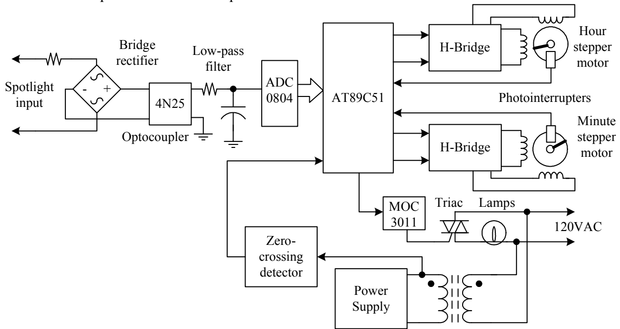
Fig. 4. Block diagram of the microprocessor-controlled grandfather clock
