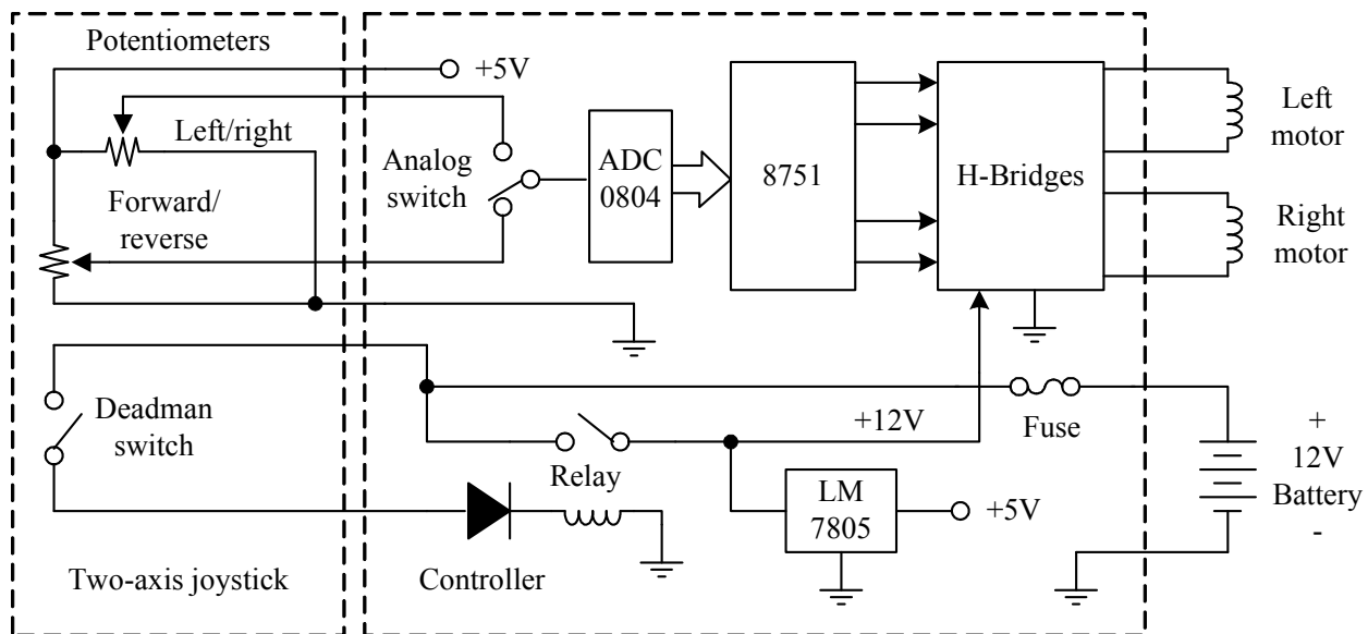
Fig. 3. Block diagram representation of the motorization of the Nutcracker sleigh.
