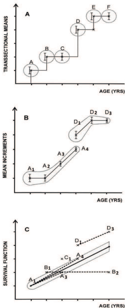
Fig. 2. Principles of trans-sectional (A) and longitudinal (B) studies as well as survival analysis (C) A. Repeated cross-sections of the means ( \pm SD) of a group of subjects (e.g. born on year A, B, C or else, for example a school grade A, B, C etc) form the mean prevalence or index curve. B. The group A is followed for three consecutive years from A 1 to A 4 and group D is followed for two years from D 1 to D 3 . The difference between step A 4 and D 1 shows the difference between longitudinal and trans-sectional analyses. C. All observations of the examinations of age cohorts (2A) and longitudinal (dotted lines) study groups (2B) are combined as a summary survival estimate (solid line) as long as information is available. There are numerous statistical methods to model this
