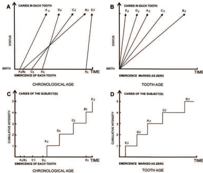
Fig. 3. The principle of time to event analysis
