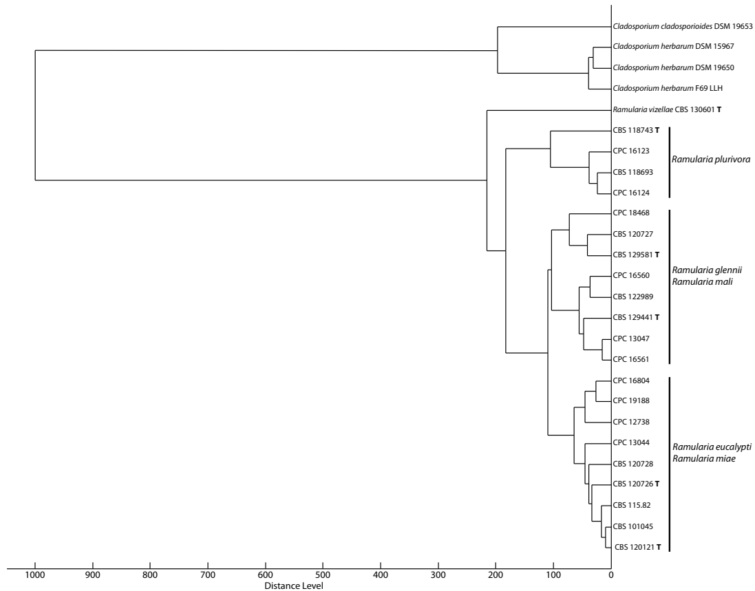
Fig. 1 PCA dendrogram based on the measured MSPs.
