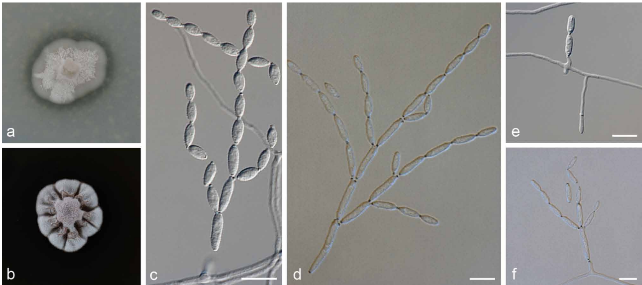
Fig. 5 Ramularia glennii (CBS 129441). a. Culture on OA; b. culture on MEA; c–f. hypha, conidiophores and conidia. — Scale bars = 10 µm.
