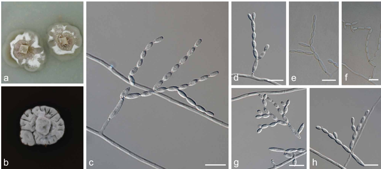
Fig. 7 Ramularia mali (CBS 129581). a. Culture on OA; b. culture on MEA; c–h. hypha, conidiophores and conidia. — Scale bars = 10 \mu m.
