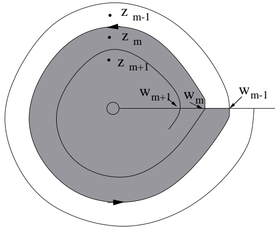
FIGURE 7. A neighborhood of the spiral. The shaded region is part of the domain of an interior differential from \{x_i, w_{m-1}\} to \{x_j, w_m\} .
