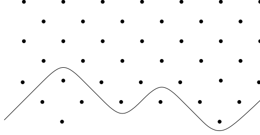
FIGURE 10. The generators of CF^+(K(13, 5), \mathbf{s}_0) . The subcomplex C_0 lies below the line, and the quotient complex CF_s^+ is above it.
