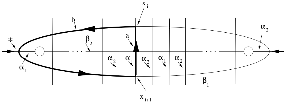
FIGURE 6. The interior region. We have drawn the case when x_i is above x_{i+1} , but the reverse may also be true.
