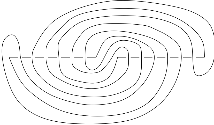
FIGURE 2. The Schubert normal form of K(7, 3)
