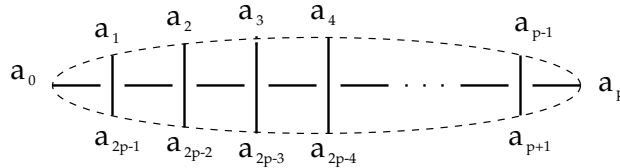
FIGURE 3. A neighborhood of an underbridge.
