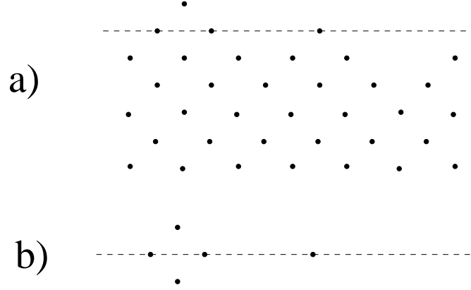
FIGURE 11. To obtain C_0 for K(13,5) , we a) truncate CF_s^- at grading -1 and b) take the union of this set and its reflection.
