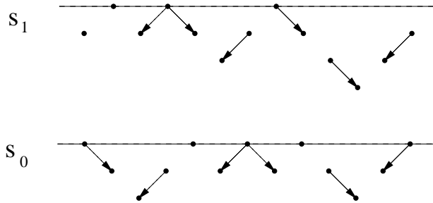
FIGURE 9. \widehat{CF}(K(13, 5), \mathbf{s}_1) and \widehat{CF}(K(13, 5), \mathbf{s}_0) . Exterior differentials are shown by dashed lines. In each case, the line of reflection is drawn in. (Compare with Figure 8b.)
