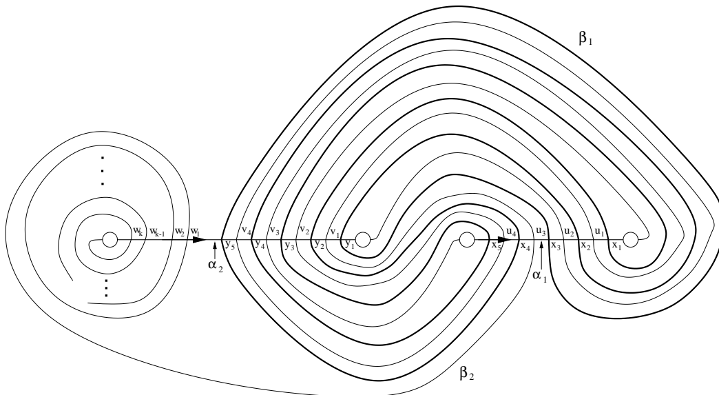
FIGURE 5. The Heegaard splitting for large n surgery on K(5, 3) . Note that for large n , \beta_2 always has many clockwise spirals, although the exact number depends on the knot.
