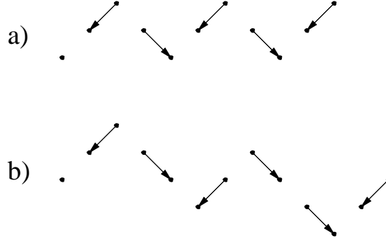
FIGURE 8. The stable complexes of a) K(11, 5) and b) K(13, 5) . The generators x_1, x_2, \dots, x_p are represented by dots, running from left to right. The grading of each generator is shown by its height, and interior differentials are indicated by arrows.
