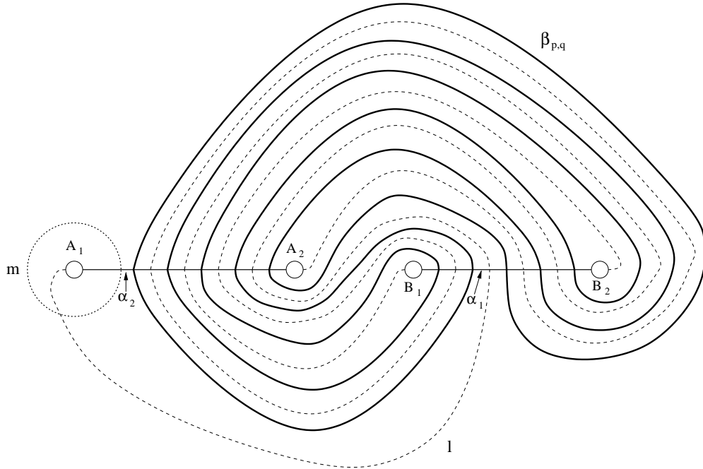
FIGURE 4. The Heegaard splitting for the complement of K(5,3) (the figure-eight knot.) The longitude and meridian are shown by dashed lines. In a general knot, the longitude will spiral around the hole labeled A_1 , so that it has intersection number zero with the class of \alpha_1 - \alpha_2 .
