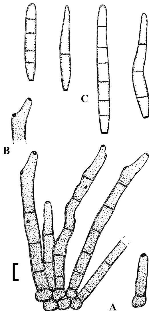
Fig. 14. Cercospora adiantigena (K(M) IMI 106709b). A. Conidiophore fascicle. B. Conidiogenous cells. C. Conidia. Bar = 10 \mu m.
