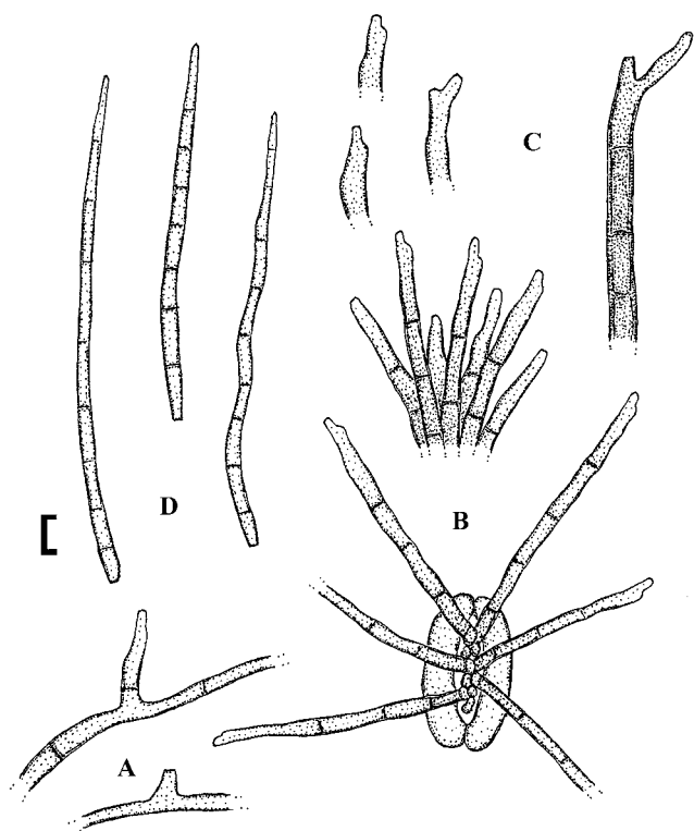
Fig. 51. Pseudocercospora pteridigena (CUP, holotype). A. Solitary conidiophores arising from superficial hyphae. B. Conidiophore fascicles. C. Conidiogenous cells. D. Conidia. Bar = 10 µm.
