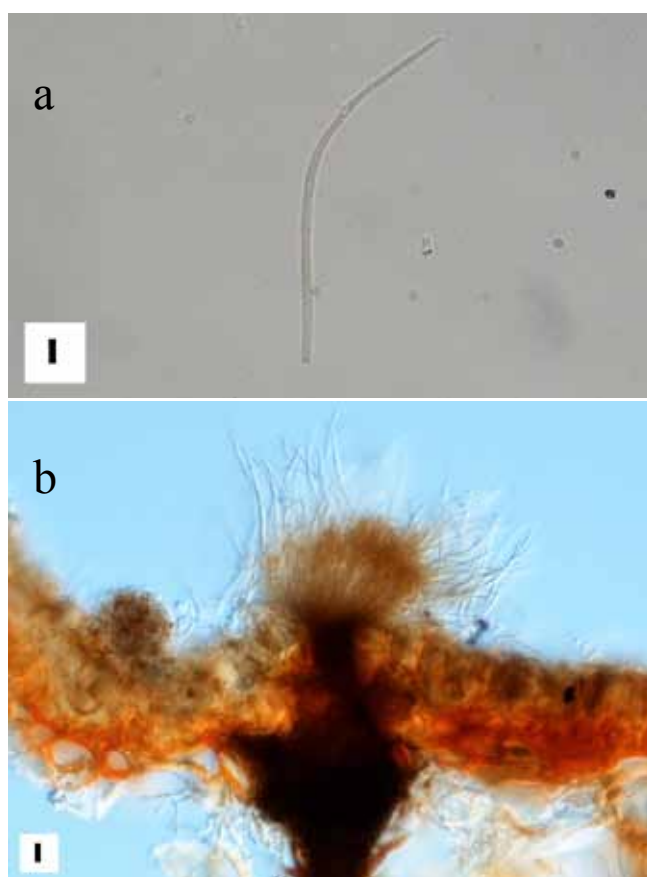
Fig. 66. Pseudocercospora sciadopytios (TFM:FPI-4757). a. Conidium (light microscopy). b. Conidiophore fascicle (light microscopy). Bars = 5 \mu\text{m} (a) and 10 \mu\text{m} (b).
