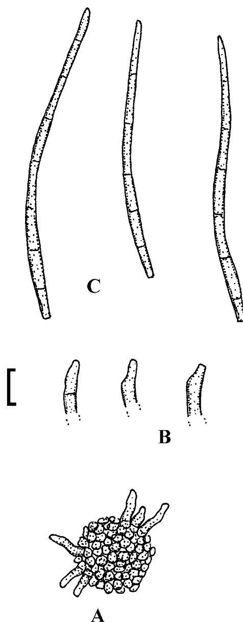
Fig. 32. Pseudocercospora christellae (MFLU10-0405). A. Conidiophore fascicle. B. Conidiophore tips. C. Conidia. Bar = 10 µm.
