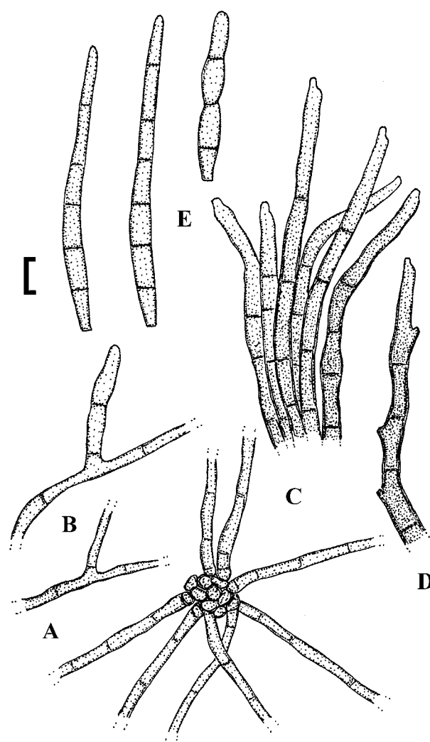
Fig. 28. Pseudocercospora adianti (HBG, lectotype). A. Superficial hyphae. B. Solitary conidiophore arising from a superficial hypha. C. Conidiophore fascicle. D. Conidiogenous cells. E. Conidia. Bar = 10 µm.
