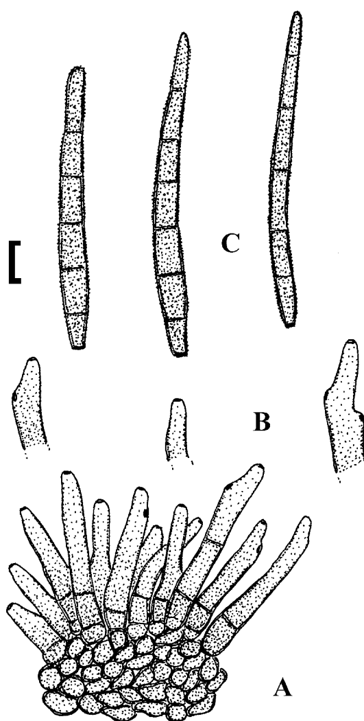
Fig. 58. Passalora sequoia (BPI 441133). A. Conidiophore fascicle. B. Conidiophore tips. C. Conidia. Bar = 10 \mu m.
