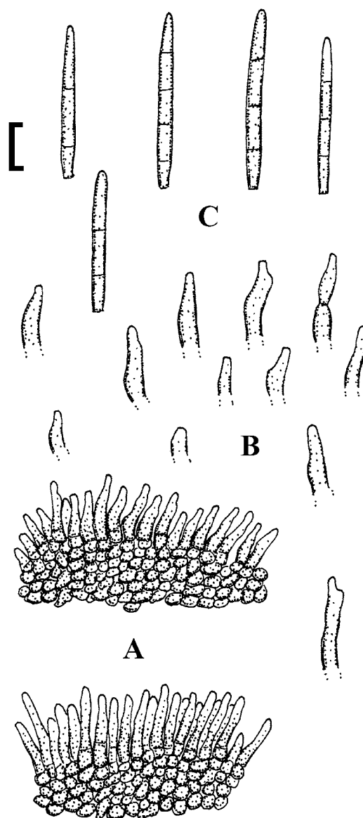
Fig. 61. Pseudocercospora exosporioides (LEP, isolectotype). A. Conidiophore fascicle. B. Conidiophores. C. Conidia. Bar = 10 \mu\text{m} .
