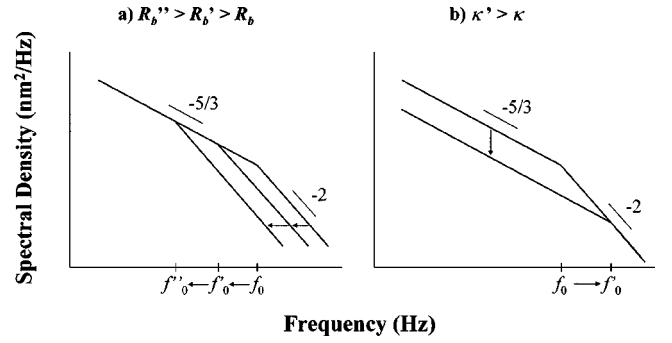
FIG. 8. Schematic dependence of the power spectrum of the out-of-plane position fluctuations in the case of a fluid membrane as a function (a) of the bead radius R_b , and (b) of the bending modulus \kappa_{\text{fluid}} .
