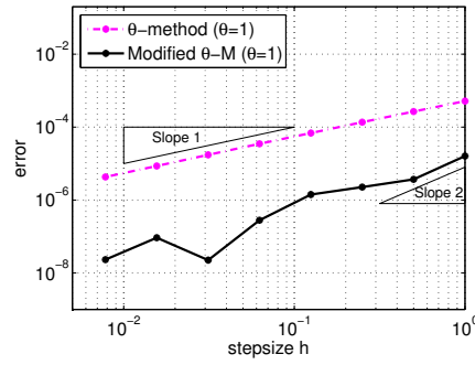
(b) Error for \mathbb{E}(X_{[1]}^2) . Very stiff case \alpha = 100 .
