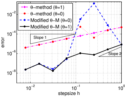
(c) Error for \mathbb{E}(X_{[1]}^2) . Stiff case \alpha = 25 .
