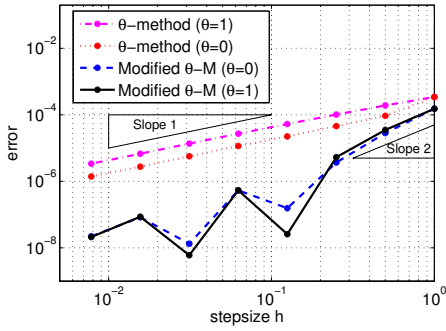
(a) Error for \mathbb{E}(X_{[1]}^2) . Nonstiff case \alpha = 1 .
