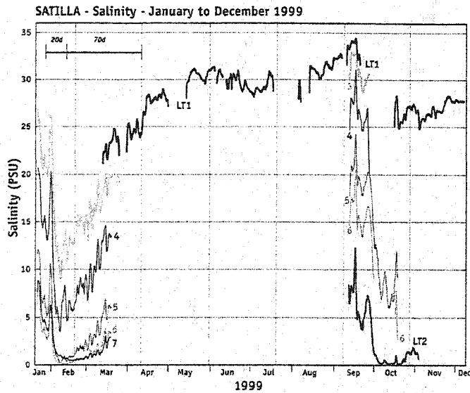
Fig. 3. Salinity measured throughout the Satilla River estuary during 1999. Tidal fluctuations have been removed by applying a low-pass digital filter to the original data. The number adjacent to the lines denote sampling locations in Figure 1. Response times of the estuary discussed in the text are shown in the upper left of the figure.
