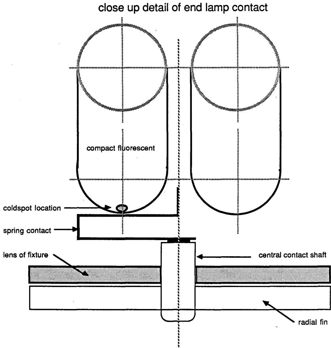
Figure 4. Detail of heat sink assembly
