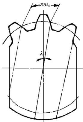
Figure 1. Helix angle of hob
