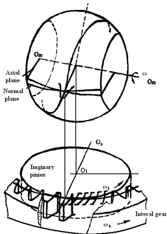
Figure 2. Principle of spherical hob
