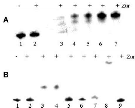
FIG. 3. EMSA with the Rv0282 upstream region. (A) Dose-response with increasing zinc concentrations. The purified Zur protein (800 ng) was incubated with the DNA fragment containing the Rv0282 upstream region (10 fmol) in the presence of increasing concentrations of ZnCl 2 in 400 μM EDTA. Binding reactions were loaded onto a nondenaturing polyacrylamide gel. Lane 1, negative control (no Zur); lane 2, no ZnCl 2 ; lane 3, 100 μM ZnCl 2 ; lane 4, 250 μM ZnCl 2 ; lane 5, 500 μM ZnCl 2 ; lane 6, 1 mM ZnCl 2 ; lane 7, 10 mM ZnCl 2 . (B) Binding of Zur to the DNA fragment containing the Rv0282 upstream region in the presence of 1 mM concentrations of different metal divalent cations. Lane 1, negative control (no Zur); lane 2, no metal cations; lane 3, Zn 2+ ; lane 4, Mn 2+ ; lane 5, Fe 2+ ; lane 6, Cu 2+ ; lane 7, Co 2+ ; lane 8, Cd 2+ ; lane 9, Ni 2+ .
